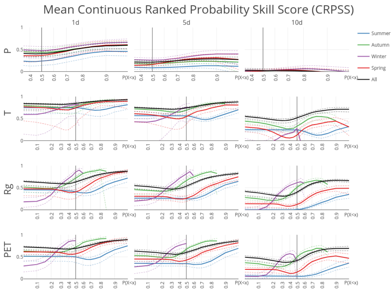
Figure 4. Continuous Ranked Probability Skill Score (CRPSS) for the four forcing variables benchmarked against sample climatology for the 148 HBV subbasins. CRPSS scores are aggregated into mean (solid), 10th and 90th percentile (dashed).
