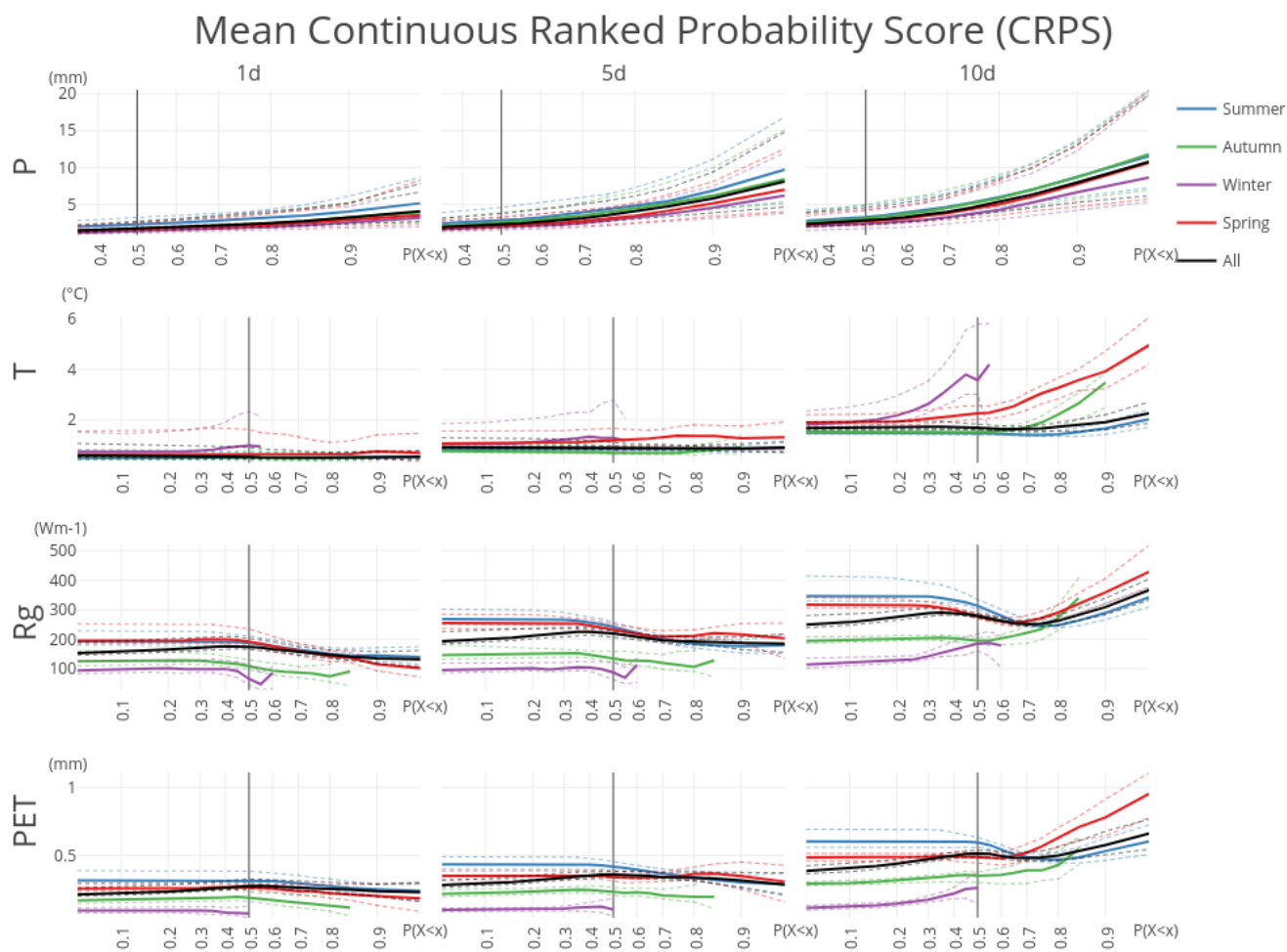
Figure 5. Continuous Ranked Probability Score (CRPS) for the four forcing variables benchmarked against sample climatology for the 148 HBV subbasins for the whole year. CRPS is aggregated into mean (solid), 10th and 90th percentile (dashed).
