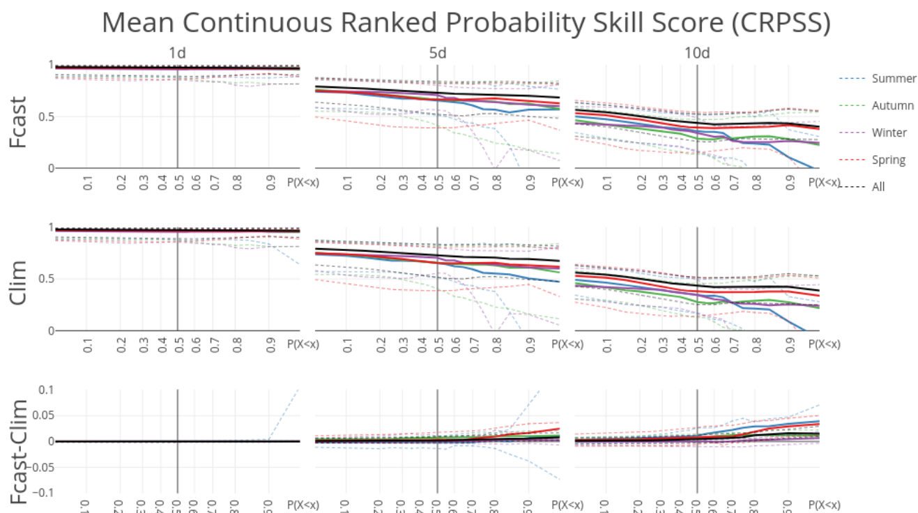
Figure 8. Continuous Ranked Probability Skill Score (CRPSS) for forecast runs (forecasted PET, climatological PET) and their difference benchmarked against model output for the 20 largest streams in the Rhine basin. CRPSS scores are aggregated into mean (solid), 10th and 90th percentile (dashed).
