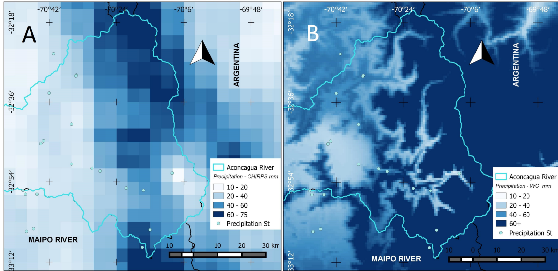
Figure 3. (A) CHIRPS precipitation for May 2009 (B) Worldclim precipitation values for May (long-term average).
