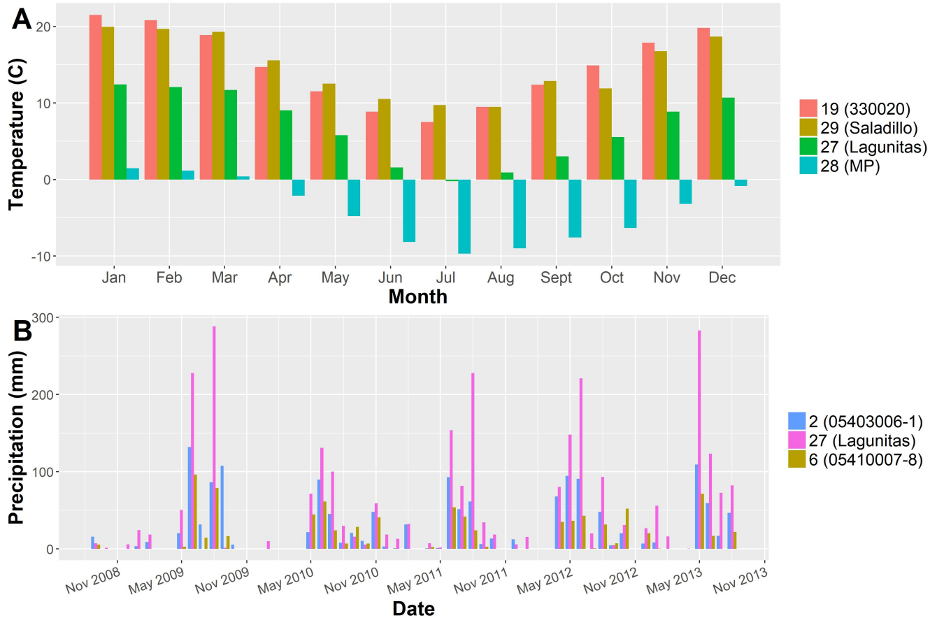
Figure 2. (A) Monthly temperature averaged over the period of analysis, 09/2008 - 08/2013, for four of the gauges in the catchment (B) Monthly precipitation in the period of analysis for three of the gauges in the catchment. The numbers in the legend correspond to those in Figure 1, while the texts in parenthesis are the names of the gauges. 330020 (527 masl), Saladillo (1580 masl), Lagunitas (2765.5 masl), MP (4250 masl), 05410007-8 (820 masl) and 05403006-1 (1290 masl).
