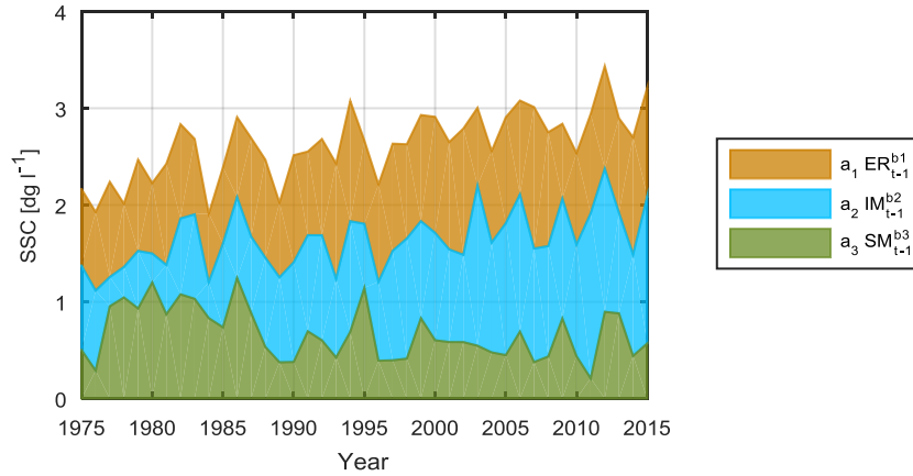
5 Figure 8: Mean annual contribution to SSC of ER_{t-1} , IM_{t-1} and SM_{t-1} simulated with the HMRC.
