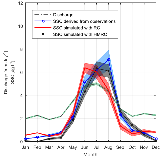
Figure 5: Mean monthly values of discharge measured at the outlet of the catchment (dash-dot grey line), SSC_t derived from observations of NTU (solid blue line with circles), SSC_t simulated with the traditional RC (solid red line), and with the HMRC
