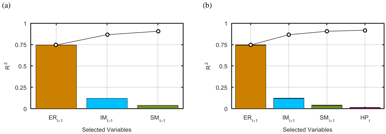
Figure 4: Results of the IIS algorithm: fraction of the variance of SSC_t explained by the selected explanatory variables, and cumulative explained variance (black line with circles) of (a) the most frequently selected model ( ER_{t-1} , IM_{t-1} , SM_{t-1} ) and (b) the most frequently selected model including hydropower releases ( ER_{t-1} , IM_{t-1} , SM_{t-1} , HP_t ).
