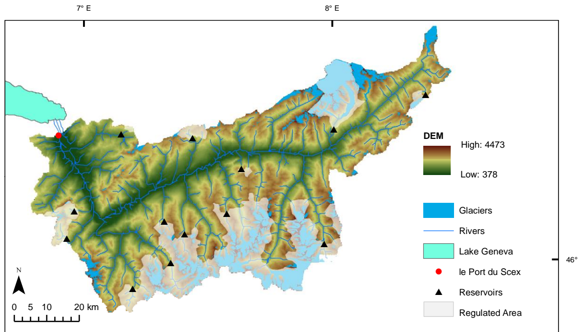
10 Figure 1: Map of the upper Rhone Basin with topography, glacierized areas and river network. The measurement station le Port– du–Scex, located just upstream the Rhone River enters the Lake Geneva, is indicated with a red marker. The main 13 reservoirs considered in this study are represented with black triangles and the regulated fraction of the catchment is highlighted with light grey shaded area.
