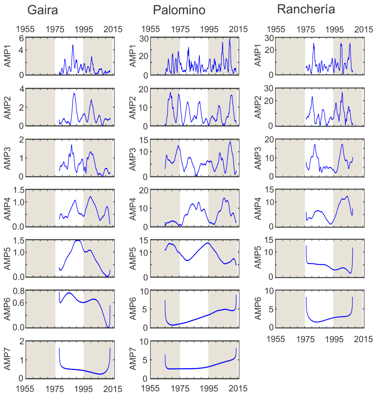
Figure 5. (Cont.) Temporal distribution of amplitudes (AMP) ( \text{m}^3 \text{s}^{-1} ) for each component (IMFs) of the Aracataca, Frío, Gaira, Palomino and Ranchería Rivers.
