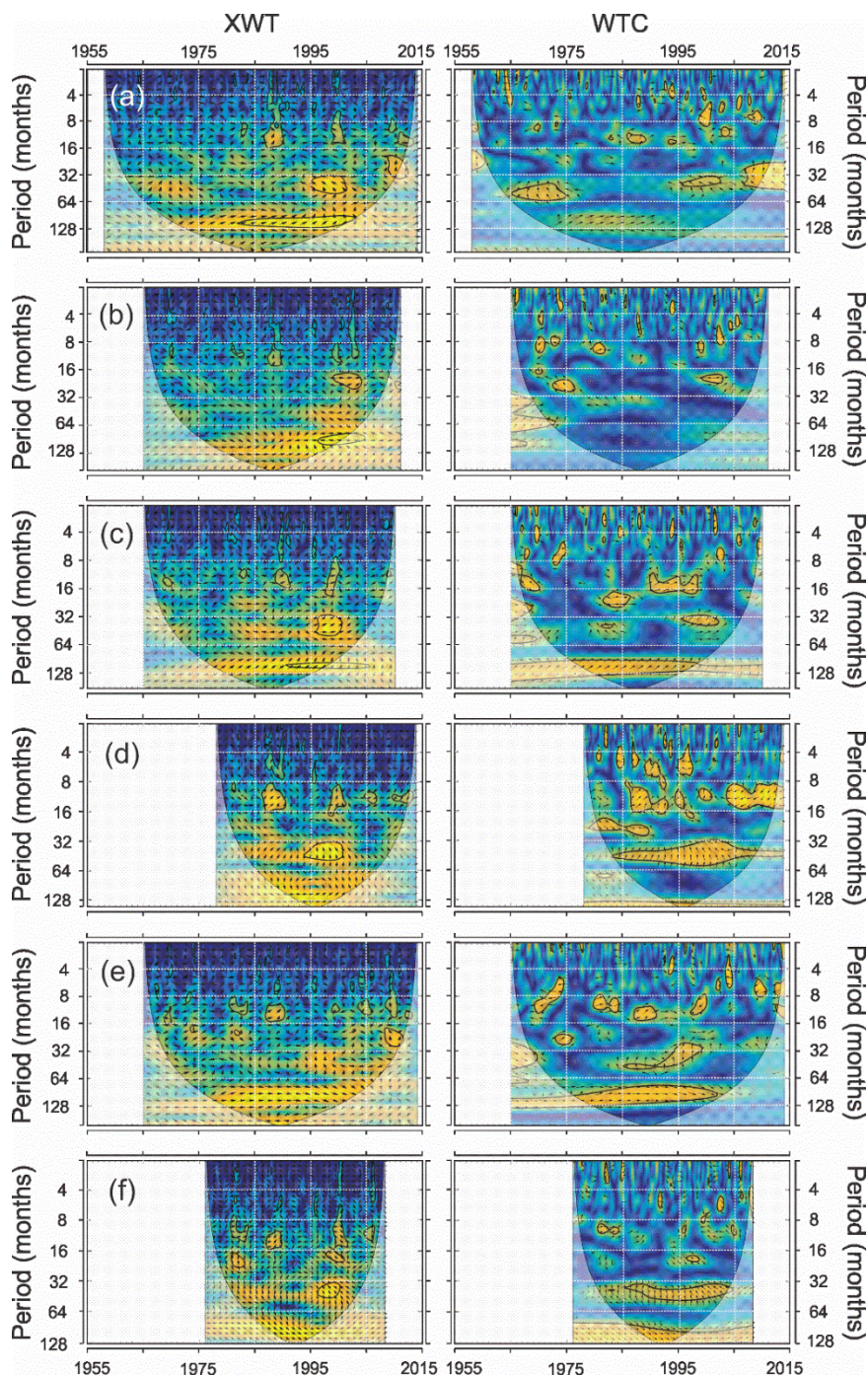
Figure 6. Cross Wavelet Transform (XWT) and Wavelet Coherence (WTC) between AMO and the (A) Fundación, (B) Aracataca, (C) Frío, (D) Gaira, (E) Palomino, and (F) Ranchería Rivers.
