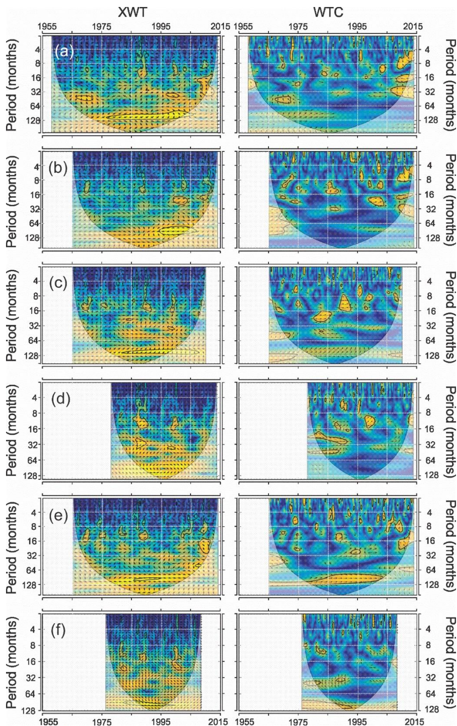
Figure 8. Cross Wavelet Transform (XWT) and Wavelet Coherence (WTC) between TNA and the (A) Fundación, (B) Aracataca, (C) Frío, (D) Gaira, (E) Palomino, and (F) Ranchería Rivers.
