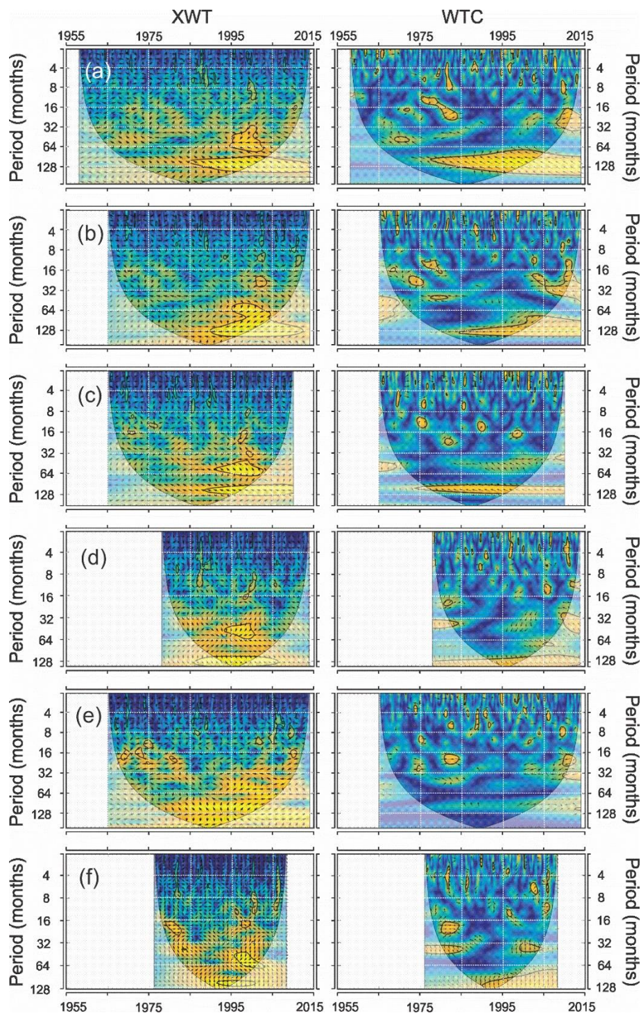
Figure 7. Cross Wavelet Transform (XWT) and Wavelet Coherence (WTC) between PDO and the (A) Fundación, (B) Aracataca, (C) Frío, (D) Gaira, (E) Palomino, and (F) Ranchería Rivers.
