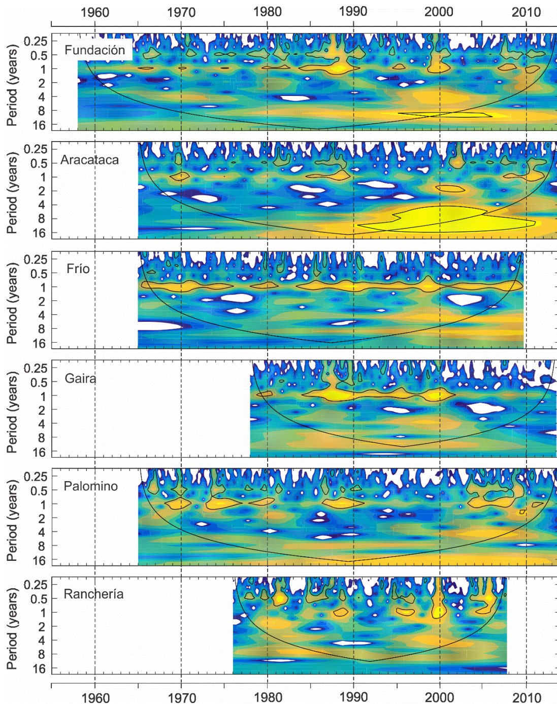
Figure 2. Continuous Wavelet transform spectrum for the Fundación, Aracataca, Frío, Gaira, Palomino and Ranchería Rivers. The dark yellow/light blue colours in the wavelet spectra correspond to high/low values of the transform coefficients (power). The thick black contour delimits the 95% confidence level against AR(1) red noise, and the cone of influence where edge effects ( T/\sqrt{2} ) are not negligible is shown as a black line.
