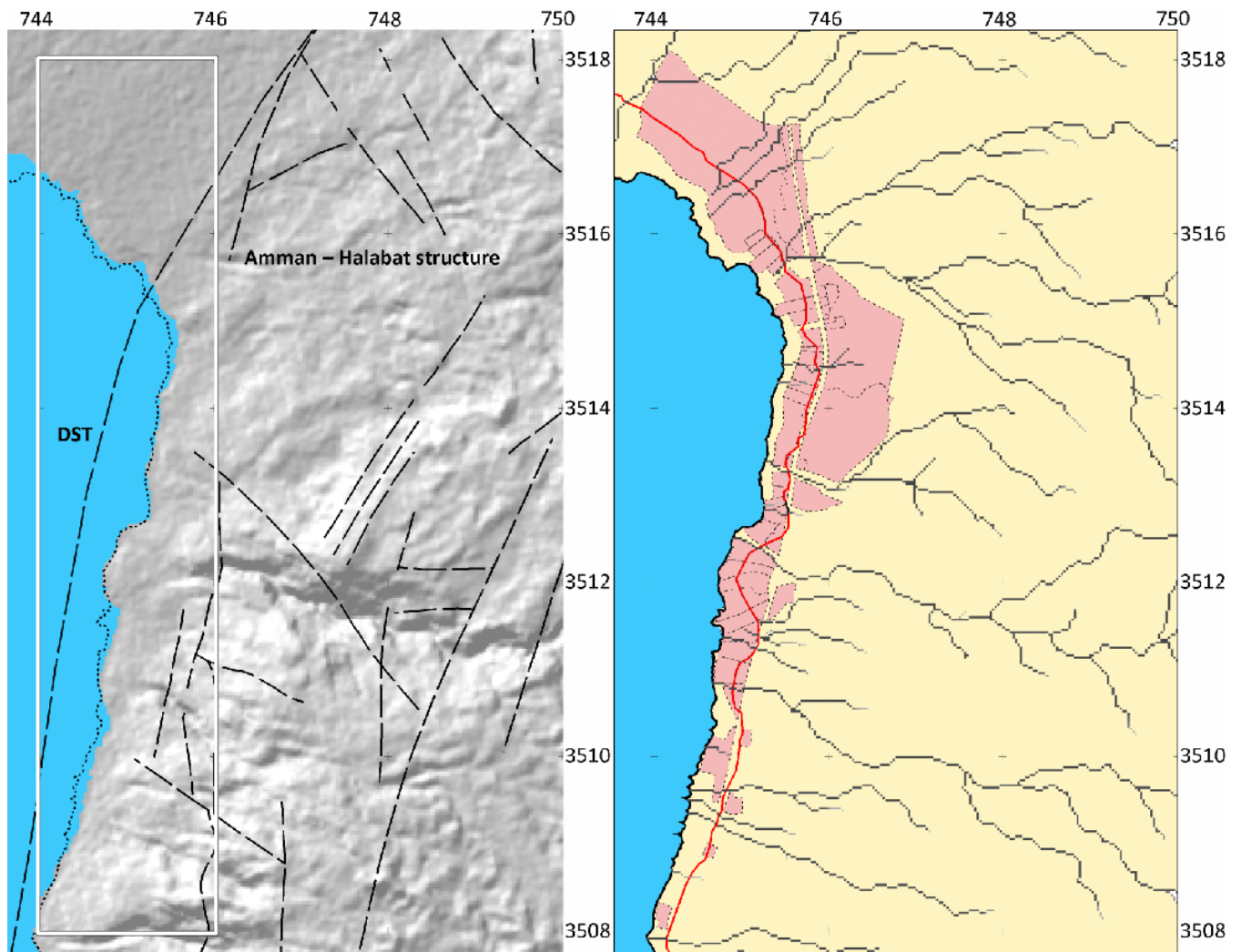
Figure 2. Hydrogeological setting of the Sweimeh area. Coordinates system: UTM 36 (km), WGS84. Left: structural features (from Al-Awabdeh, 2015). The Dead Sea Transform (DST) crosses the study area of interest (white rectangle). The black dotted line is the coastline in 2018. The hill shade relief derived from the SRTM Digital Elevation Model shows the coastline in February 2000. Right: the red line shows the coastline in 1959. The pink colour represents the cadastral parcels that are either already built-up or that are selected for future urban development. The black lines represent the thalwegs network.
