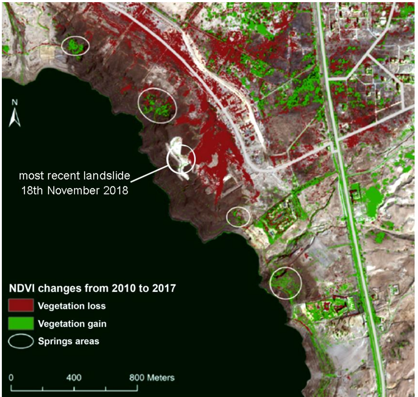
Figure 7. Vegetation change detection map obtained from NDVI difference between 2010 to and 2017 in the north-eastern part of the study area. The white circles highlight the areas along the coastline where new springs appeared in correspondence of vegetation gain along the coastline .
