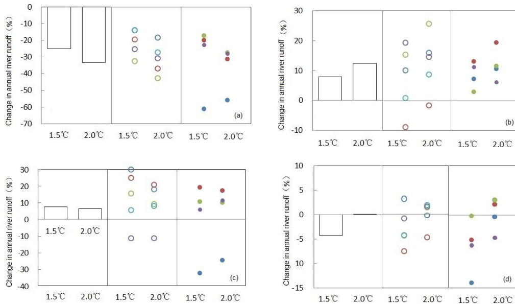
5 Figure 2. Changes in simulated annual river runoff: (a) Shiyang River, (b) Chaobai River, (c) Huaihe River, and (d) Fujiang River under 1.5 °C and 2 °C global warming. (Baseline: 1976–2005; columns represent the simulated river runoff for all combined scenarios; hollow circles colored dark blue, red, green, blue, and purple represent the GCMs: GFDL, HaDGem, IPSL, MIROC, and NorESM, respectively; solid circles colored dark blue, red, green, and purple represent the RCPs: RCP2.6, RCP4.5, RCP6.0, and RCP8.5, respectively).
