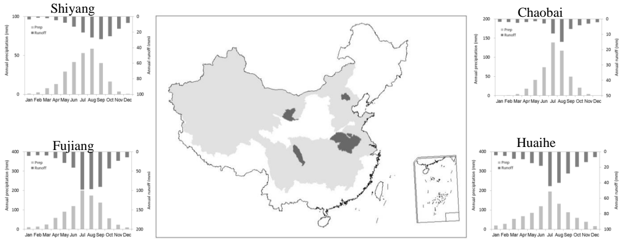
Figure 1. Locations and average monthly precipitation/runoff of the four selected basins in China.
