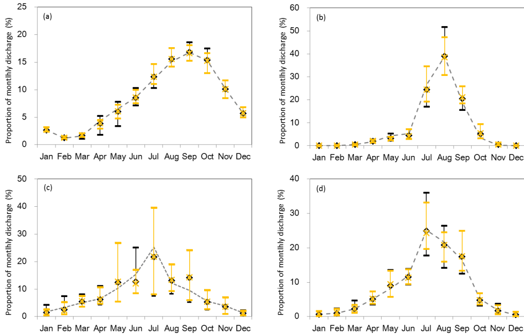
5 Figure 3. Simulated percentage changes in proportion of monthly river runoff: (a) Shiyang River, (b) Chaobai River, (c) Huaihe River, and (d) Fujiang River under 1.5 °C and 2.0 °C global warming. (Baseline: 1976–2005; bars colored black and yellow show the maximum and minimum values of all simulated monthly runoff for all combined climate change scenarios under 1.5 °C and 2.0 °C global warming; black diamonds and yellow crosses represent the mean values for monthly runoff under 1.5 °C and 2.0 °C global warming).
