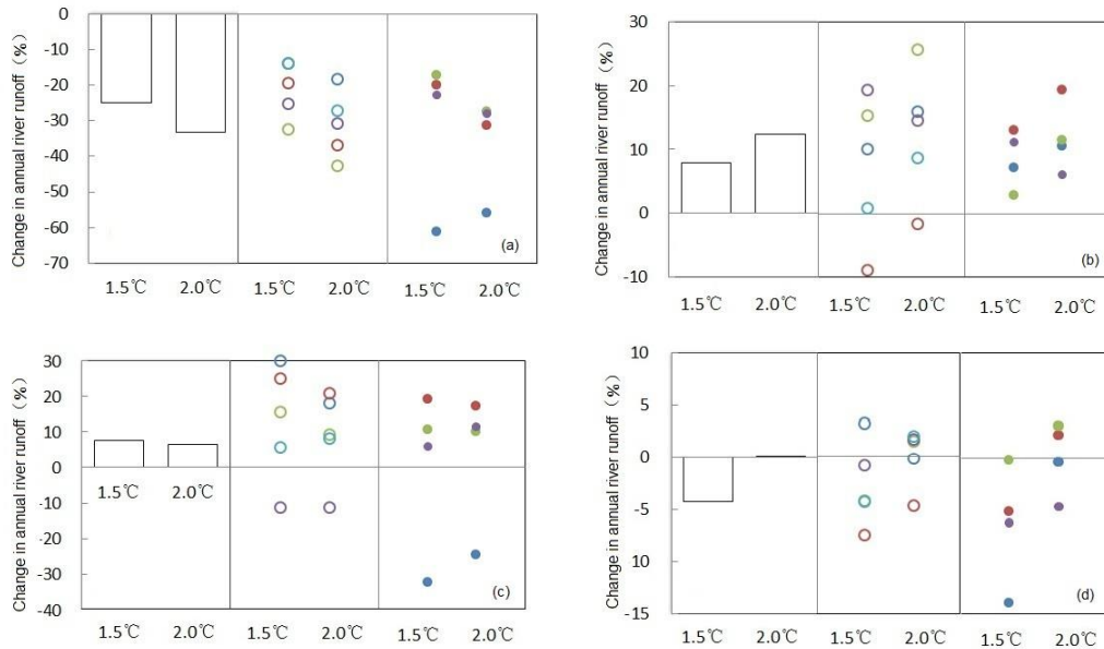
20 Figure 2. Changes in simulated annual river runoff: (a) SYR, (b) CBR, (c) HHR, and (d) FJR under 1.5 °C and 2 °C global warming. (Baseline: 1976–2005; columns represent the simulated changes in mean annual river runoff for all combined scenarios of GCMs and RCPs ; hollow circles colored dark blue, red, green, blue, and purple represent the changes in mean annual runoff simulated by five GCMs: GFDL-ESM2M, HaDGem2, IPSL_CM5A-LR, MIROC-ESM-CHEM, and NorESM1-M, respectively; solid circles colored dark blue, red, green, and purple represent the changes in mean annual runoff simulated under four RCPs: RCP2.6, RCP4.5, RCP6.0, and RCP8.5, respectively).
