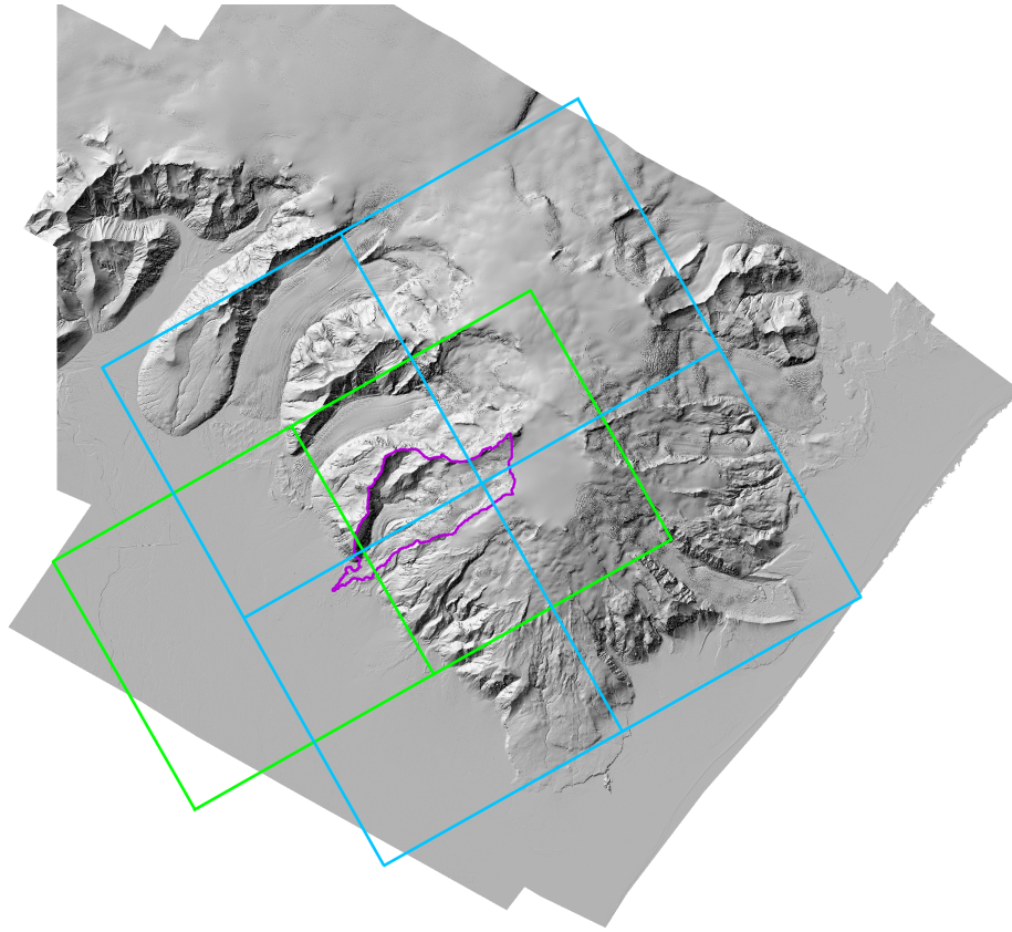
Figure A1. EURO-CORDEX 0.11^\circ RCM grid lines. RCM nodes are situated at grid line intersects. All RCMs utilise the green grid except for REMO2009 which uses the blue grid.
