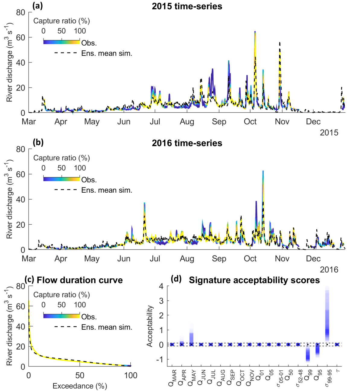
Figure 4. Capture ratio projected onto observed river discharge data during evaluation period for 2015 (a); 2016 (b); and over the FDC (c). The weighted ensemble mean simulation is shown as a black dash. Also shown are the range of acceptability scores for each of the available river discharge signatures over the evaluation period (d). Acceptable simulations in (d) are those contained within the black dash lines.
