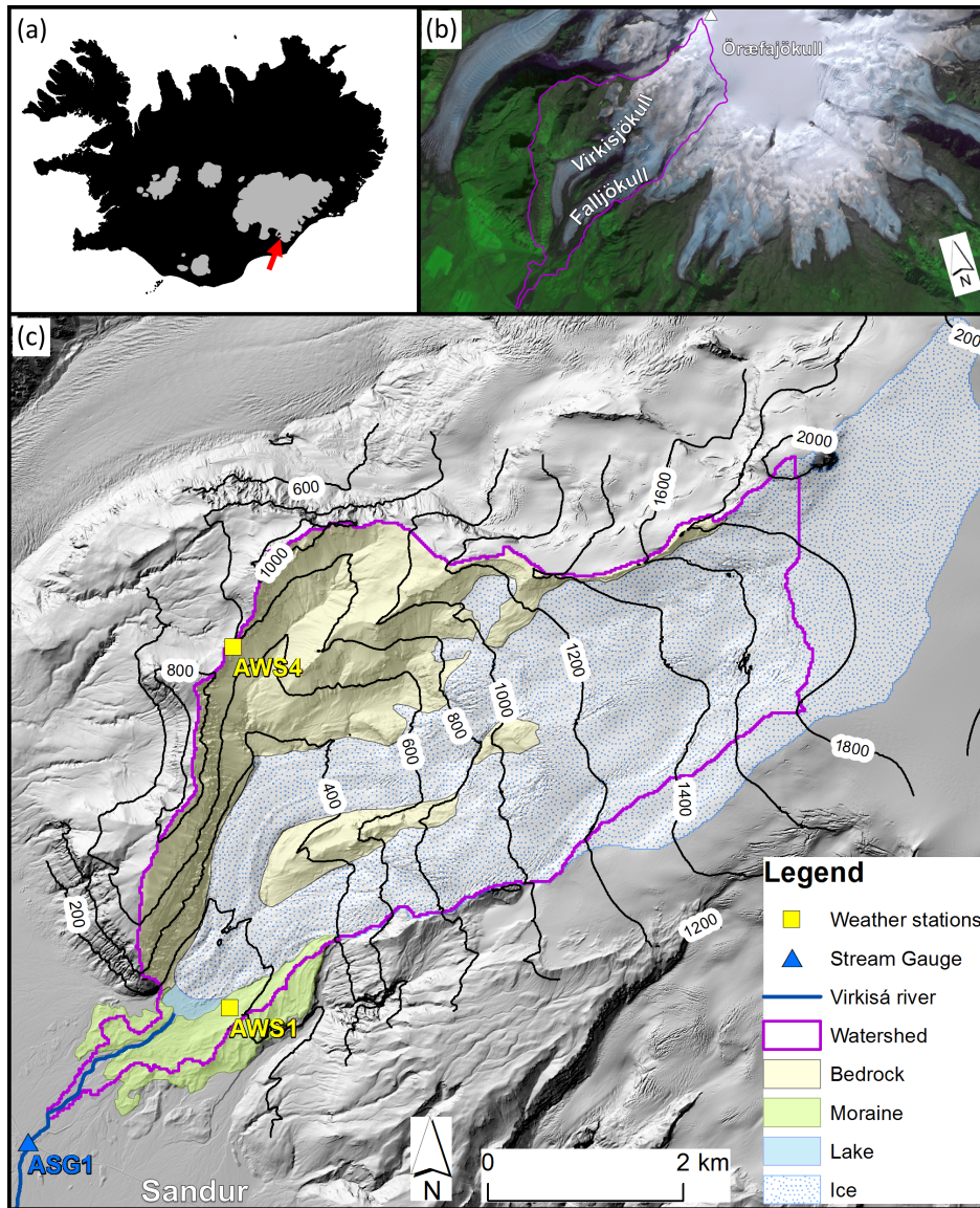
Figure 1. Location of Virkisá river basin in Iceland with glaciated areas highlighted in grey (a); on Öraefajökull (b); and detailed topographical map of basin including major land surface types and meteorological and stream gauging stations (c).
