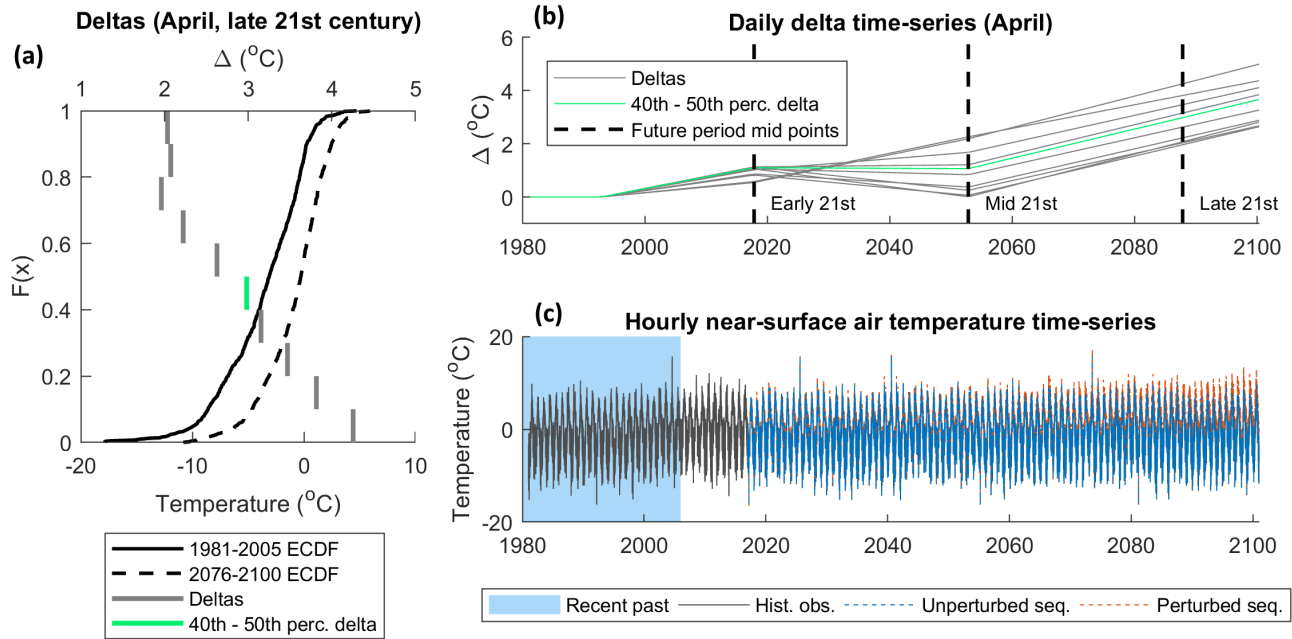
Figure 3. Example of advanced delta-change approach when applied to near surface air temperature data based on the RCP8.5 projections using the CNRM-CM5 GCM and CCLM4-8-17 RCM. Deltas (grey bars) derived from ECDFs (black curves) for April in late 21st century (a); Daily delta time-series for each section of the April ECDFs (green line represents 40th - 50th percentile section) (b); Initial and perturbed future temperature time-series when deltas for all months and ECDF sections are applied (c).
