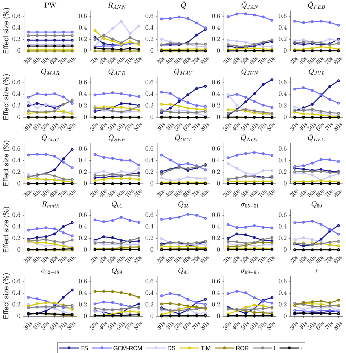
Figure D1. Effect size of all main effects, interactions and remaining error on projected decadal changes in the 25 river discharge signatures for all future time-slices centred on the 2030s to the 2080s.
