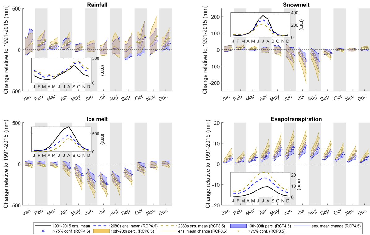
Figure 11. Projections of monthly mean runoff components including rainfall (a), snowmelt (b), ice melt (c) and evapotranspiration (d) for RCP4.5 (blue) and RCP8.5 (yellow). For each month, the trajectory of the ensemble mean change over the 21st century time-slices (2030s to 2080s) relative to the reference period (1991-2015) is shown by the solid coloured lines. These lines are marked for each time-slice where there is \geq 75\% confidence in the direction of change. They are bounded by the 10th and 90th percentiles of the projections (bands). Inset in each plot are ensemble mean monthly runoff volumes averaged over the reference period (black solid line) and 2080s (dashed lines).
