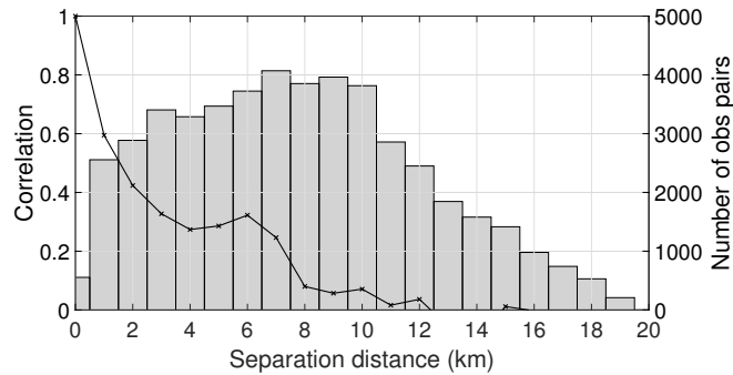
Figure 2. Estimated SAR WLO error correlations (black line) and number of samples (bars) used for the calculation. Estimated error standard deviation 54cm.
