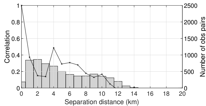
Figure 4. Estimated SAR WLO error correlations (black line) and number of samples (bars) used (bin width = 1km). East domain. Estimated error standard deviation 43cm.
