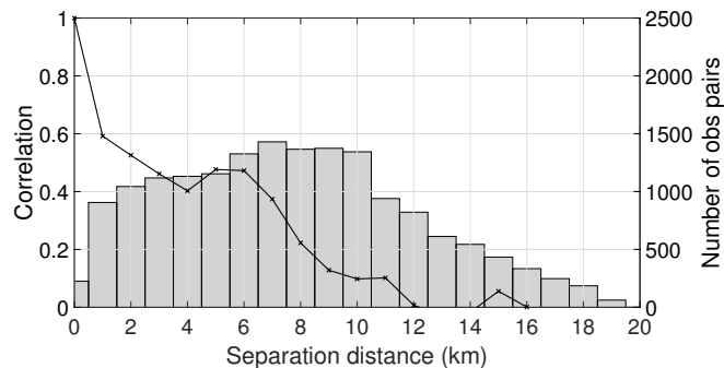
Figure 7. Estimated SAR WLO error correlations (black line) and number of samples (bars) used (bin width = 1km). 2nd and 4th December. Estimated error standard deviation 57cm.
