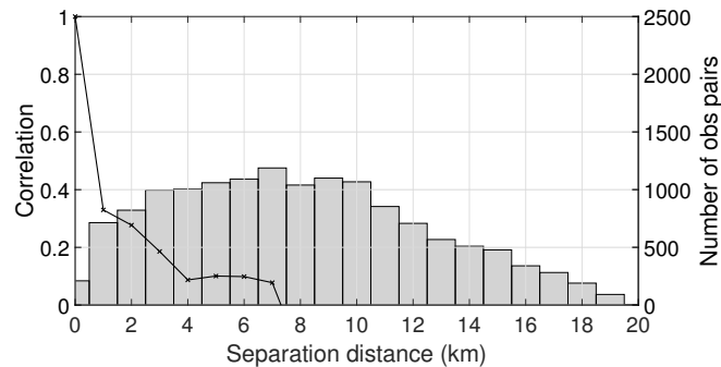
Figure 6. Estimated SAR WLO error correlations (black line) and number of samples (bars) used (bin width = 1km). 30th November and 1st December. Estimated error standard deviation 43cm.
