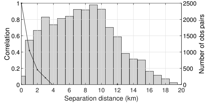
Figure 5. Estimated SAR WLO error correlations (black line) and number of samples (bars) used (bin width = 1km). 27th, 28th 29th November. Estimated error standard deviation 53cm.
