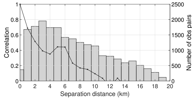
Figure 3. Estimated SAR WLO error correlations (black line) and number of samples (bars) used (bin width = 1km). West domain. Estimated error standard deviation 58cm.
