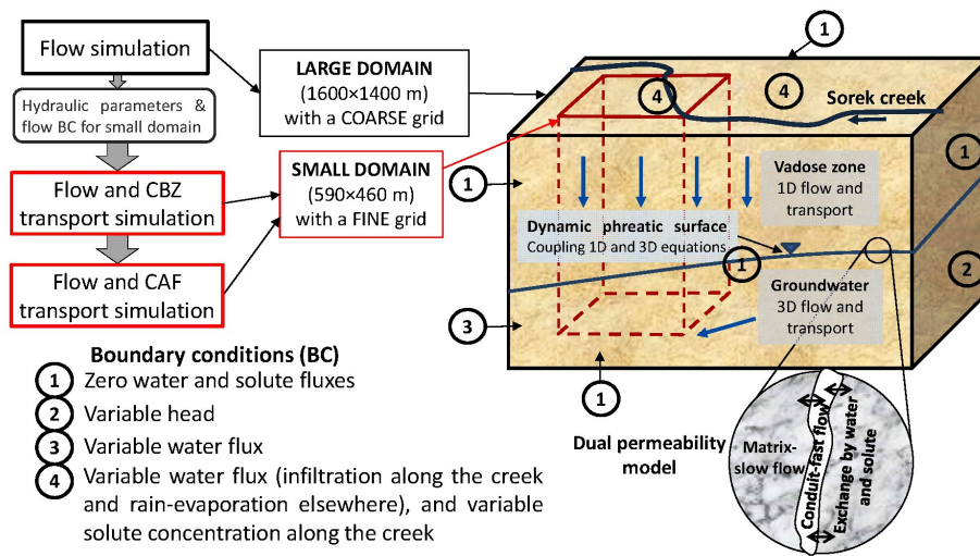
Fig. 2. Model conceptual sketch
