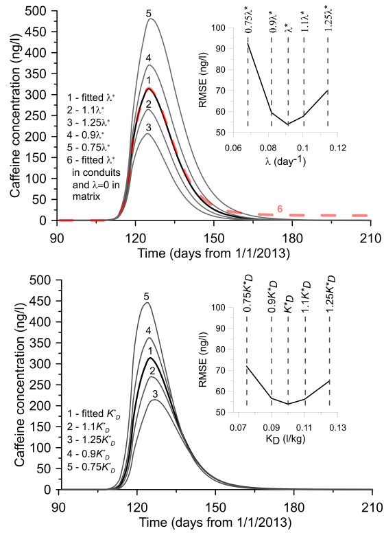
Fig. 5. Simulated CAF sensitivity to parameters changes (A) the degradation rate and (B) the distribution coefficient. The insets show the effect of parameters on RMSE.
