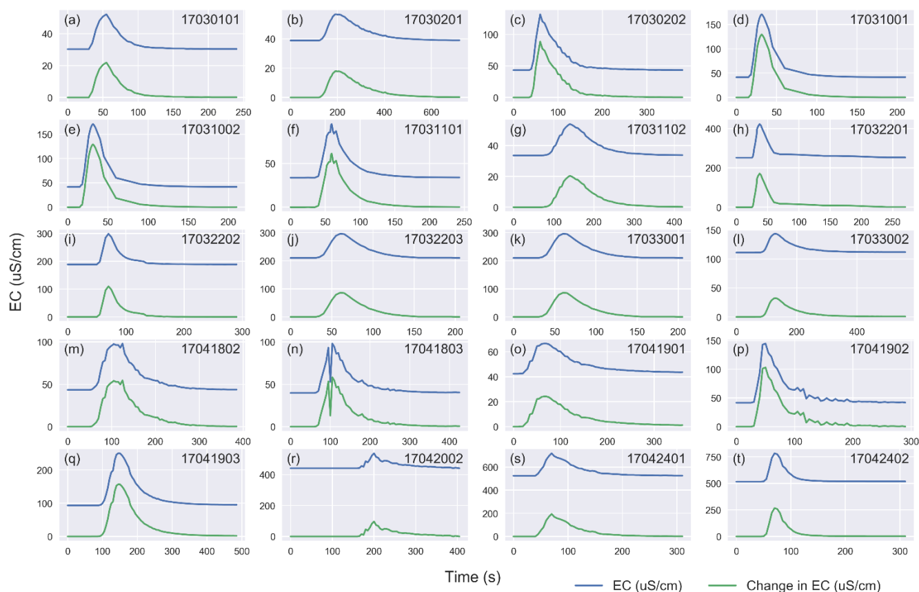
Figure 2: Plots of EC ( \mu\text{S cm}^{-1} ; blue trace) and change in EC ( \mu\text{S cm}^{-1} ; green trace) as a function of time (s) for the 20 salt dilution evaluation measures. Measurement ID (Msmt ID; Table 1) shown at the top right of each subplot (i.e. a through t).
