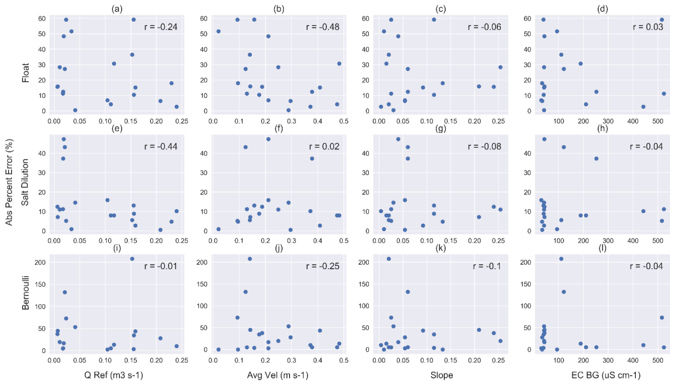
Figure 4: Scatter plots between reference flow (Q Ref; \text{m}^3 \text{s}^{-1} ), average water velocity (Avg Vel; \text{m s}^{-1} ), slope, and background EC (EC BG; \mu\text{S cm}^{-1} ) and absolute value (Abs) of percent errors for float, salt dilution, and Bernoulli. Pearson's r values shown on the upper right of each subplot (i.e. a through l).
