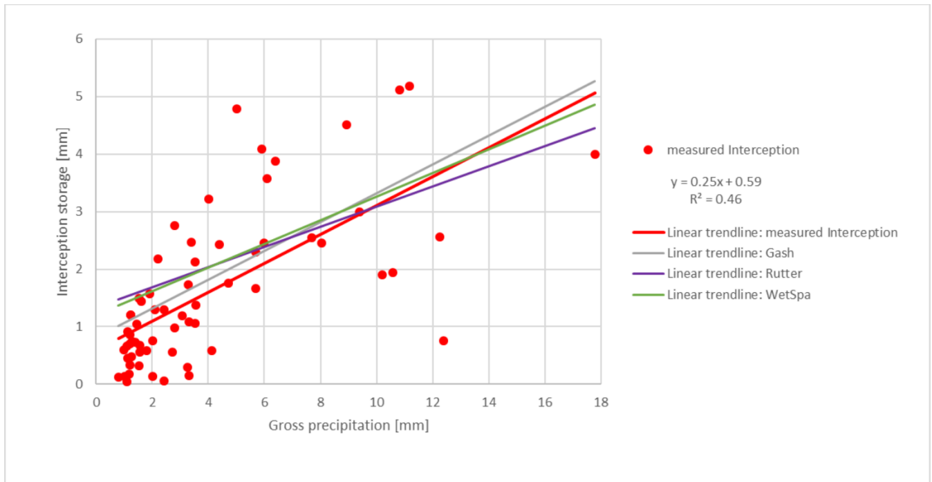
20 Figure 5: Interception storage vs gross precipitation for all events for both trees.
