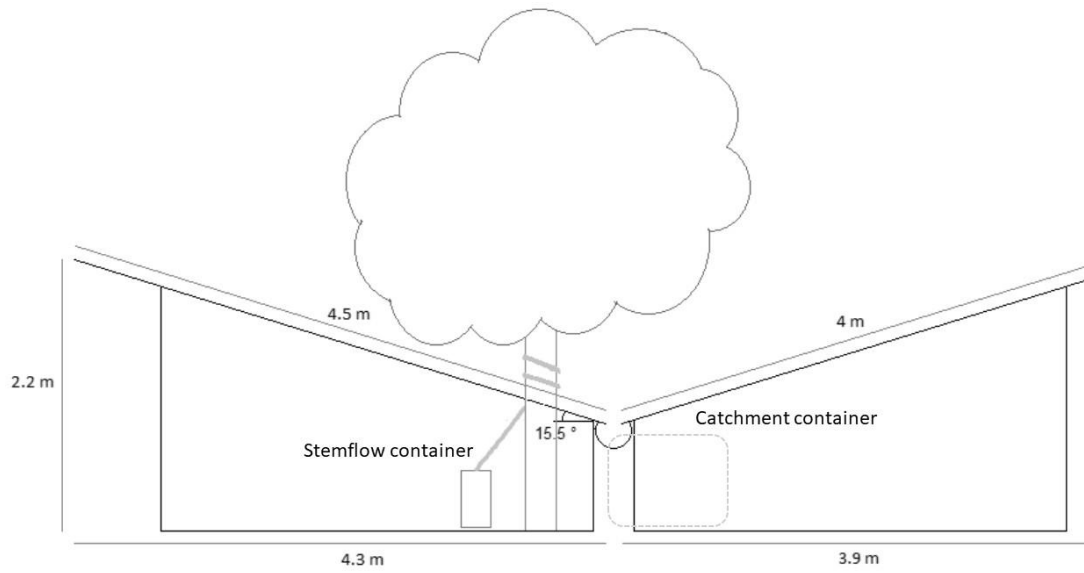
Figure_33: Schematic representation of the V-catchment construction.
