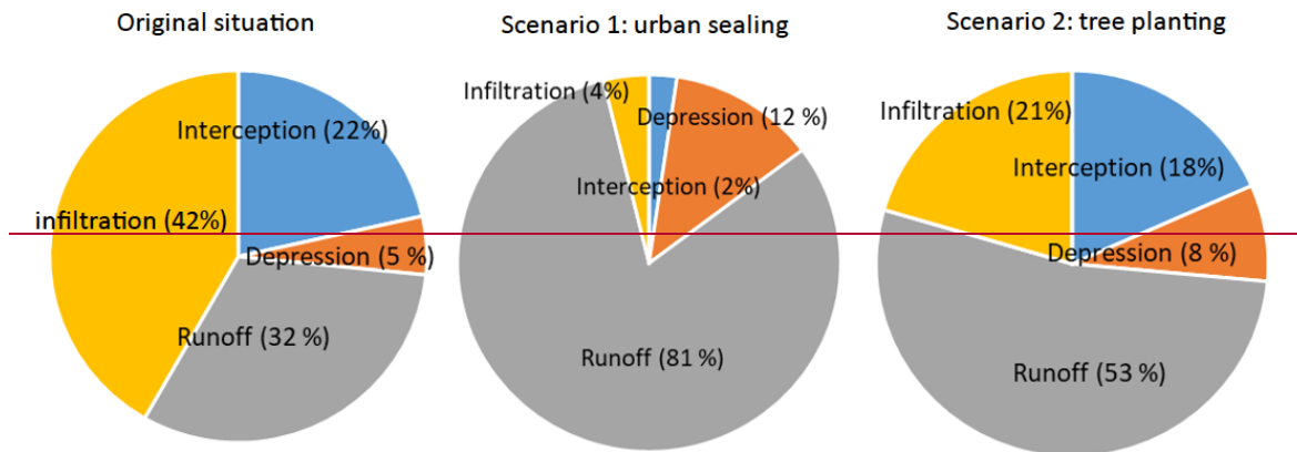
Figure 14: Yearly (2015) surface water balance [% rainfall] for the different scenario's.
