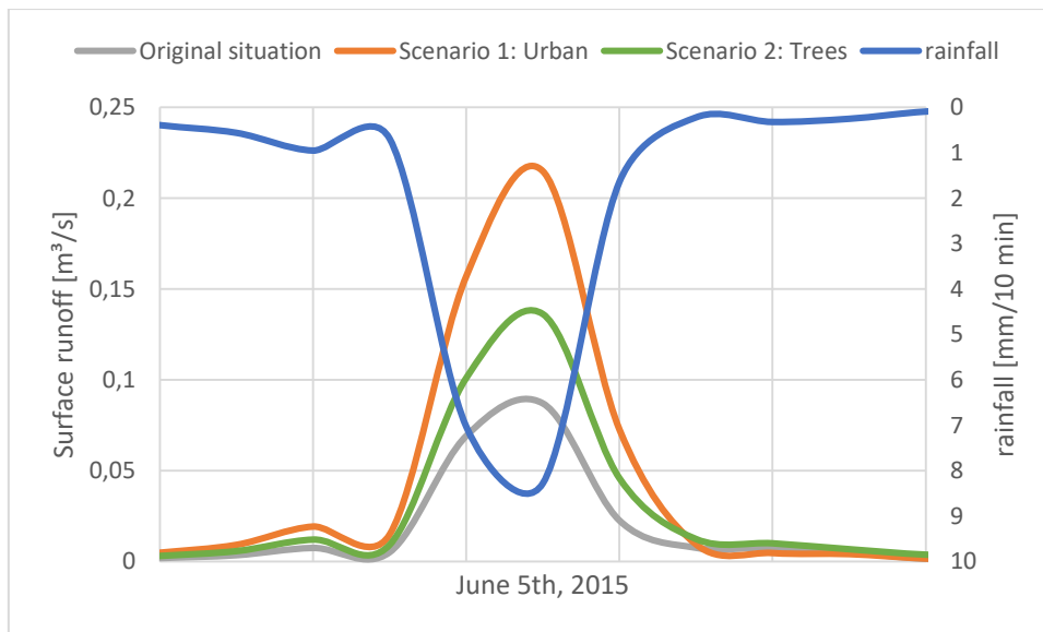
Figure 15: hydrographs for 2015 event (return period 2 years Ucele).
