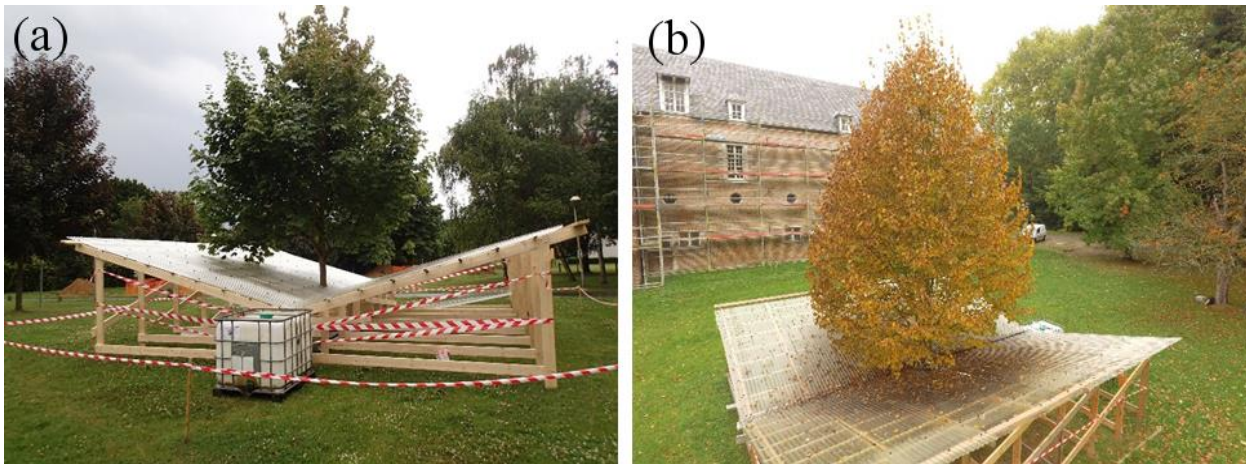
Figure_44: Images of the V-catchment under the Norway maple (a) [picture: 30 July 2015] and small leaved lime (b) [picture: 21 October 2016].
