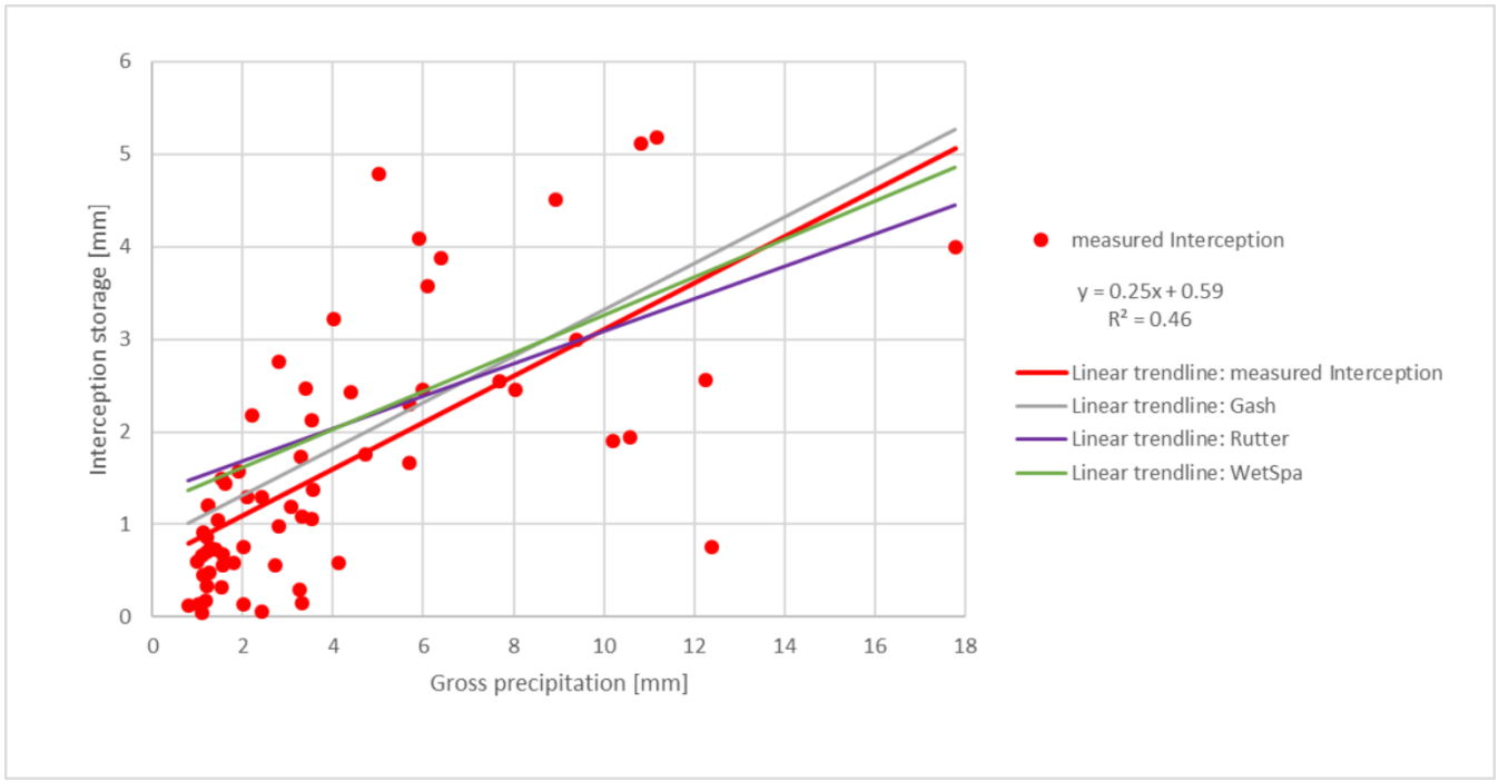
Figure-512: Interception storage vs gross precipitation for all events, for both trees.
