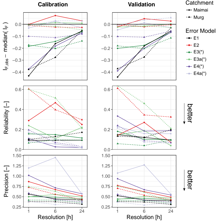
Figure 3. Performance of the error models w.r.t. flashiness index, reliability and precision for both catchments and all temporal resolutions. P_{err} was smoothed (*) exclusively for hourly data in the Maimai catchment.
