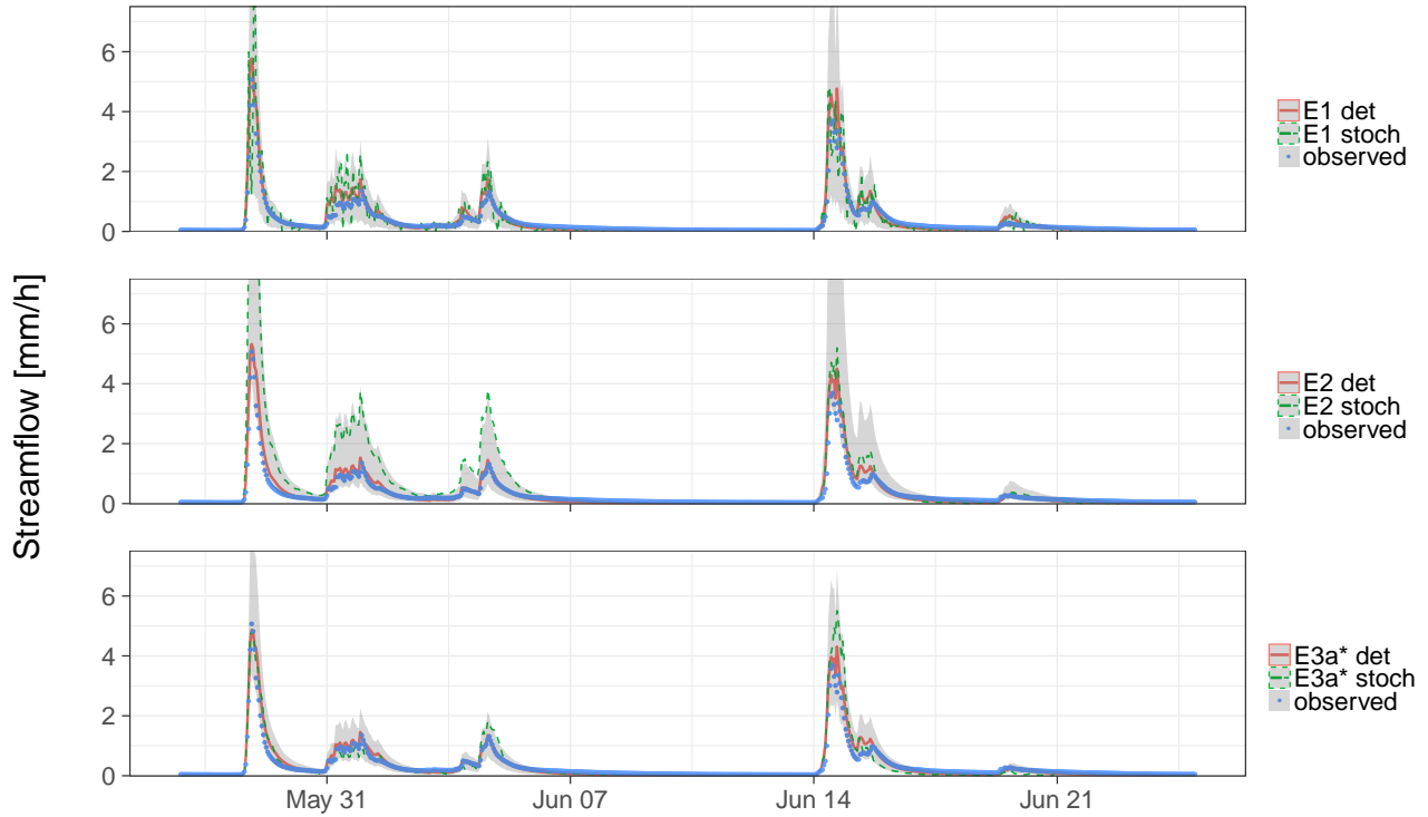
Figure 5. Streamflow predictions with hourly resolution in the Maimai creek in a part of the validation period (1993). Deterministic predictions with the parameter values at the maximum posterior density are shown together with the 90%-confidence bands and one single stochastic streamflow realisation for each of the error models.
