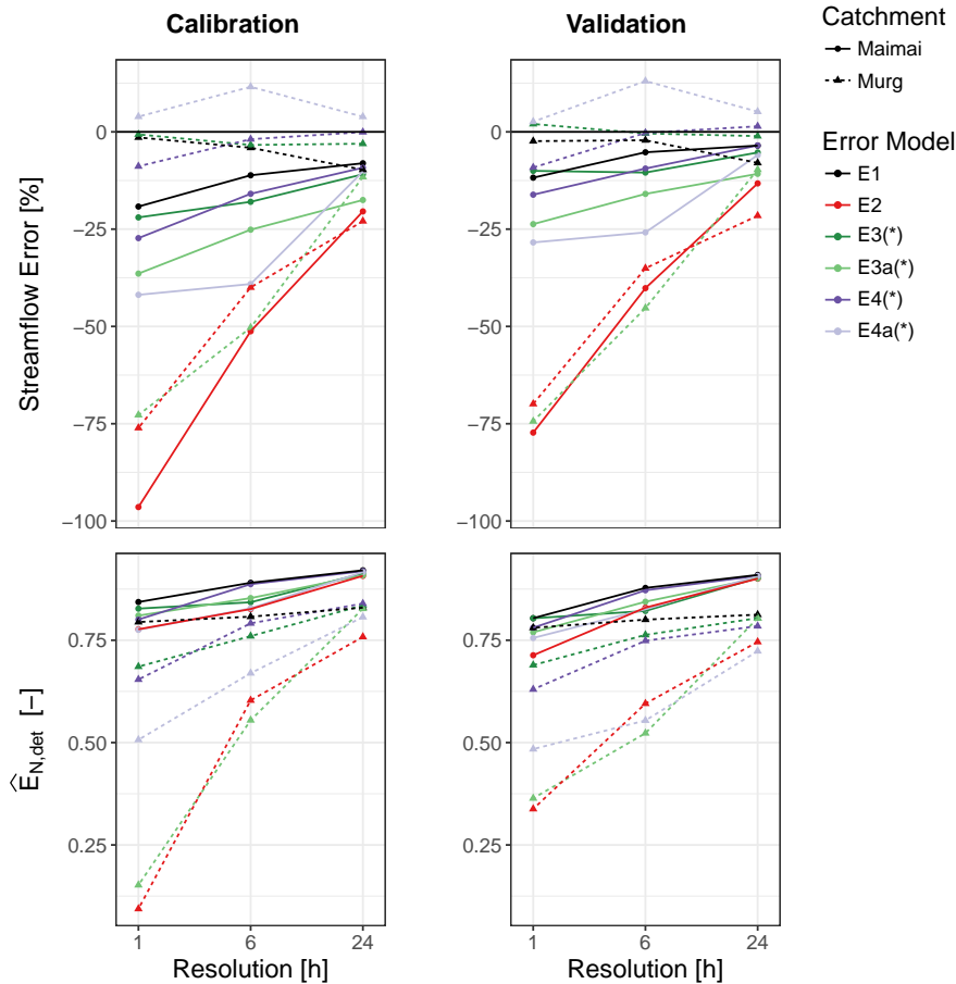
Figure 4. Performance of the error models in terms of the relative cumulative error in streamflow, \Delta_Q , and the Nash-Sutcliffe Efficiency, \hat{E}_{N,\text{det}} , for both catchments and all temporal resolutions. P_{\text{err}} was smoothed (*) exclusively for hourly data in the Maimai catchment.
