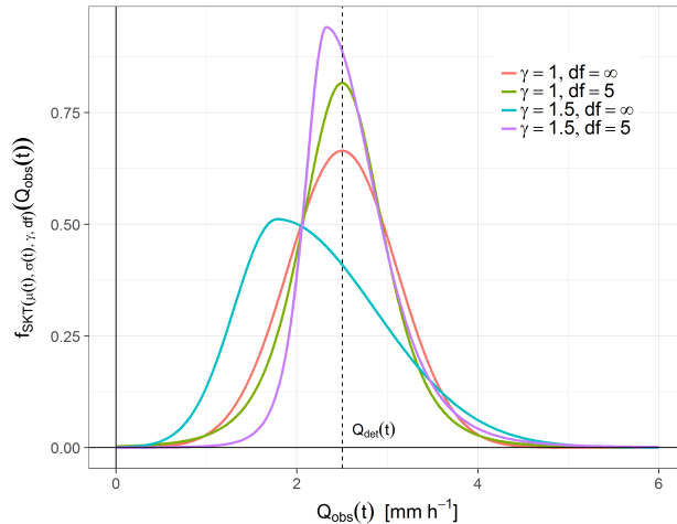
Figure 1. Example of skewed Student’s t -distributions with E[D_Q] = Q_{\text{det}}(t) = 2.5 \text{ mm h}^{-1} and standard deviation \sigma_{D_Q}(t) = 0.6 for different values of skewness, \gamma , and kurtosis, df .
