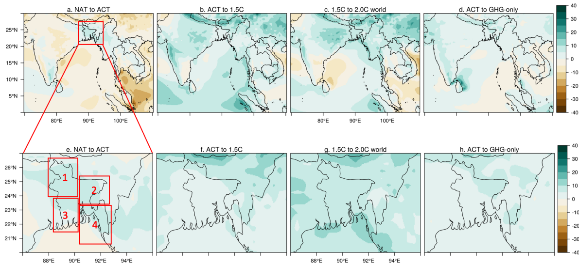
Figure 3: Same as Fig. 2, but for JJAS rainfall dPercent. The four boxes (1-4) of the panel e represent the four sub-regions of Bangladesh. This figure shows that the apparently non-linear response between panels of a, b, and c (or, e, f, g) can be explained by the response for GHG-only (anthropogenic aerosols reduced to pre-industrial levels) in panel d (or, h).
