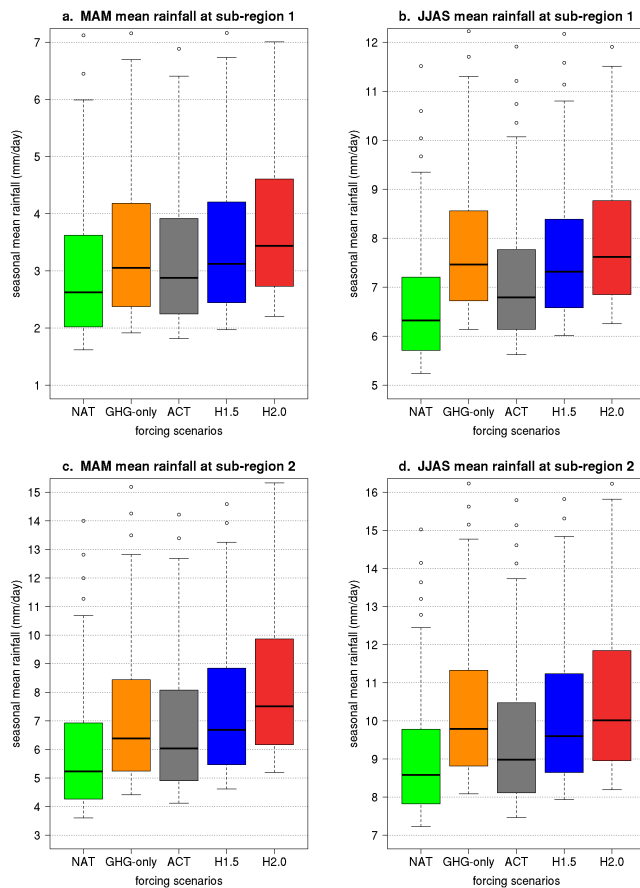
Fig. 3. AC3 c: Seasonal mean rainfall in MAM (left column) and JJAS (right column) over the sub-regions 1 and 2 (top and bottom row) of Bangladesh.
