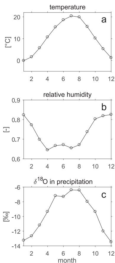
Figure 3. Long-term mean monthly air temperature (a), relative humidity (b) and oxygen isotopic composition in precipitation (c) for the station Vienna Hohe Warte, Austria
