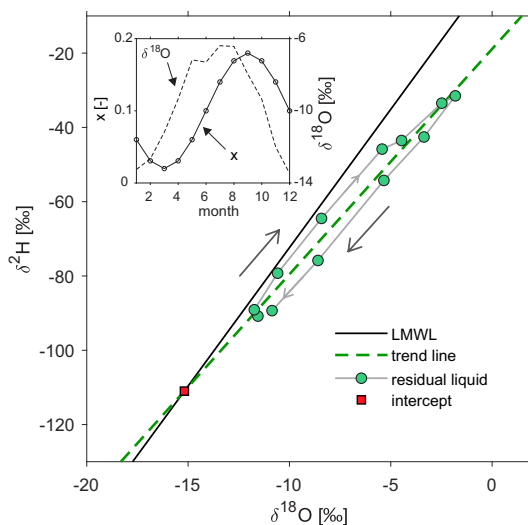
Figure 6. Hysteretic pattern arising in the computed residual liquid when the seasonality of source water composition and that of evaporation (inset) are shifted.
