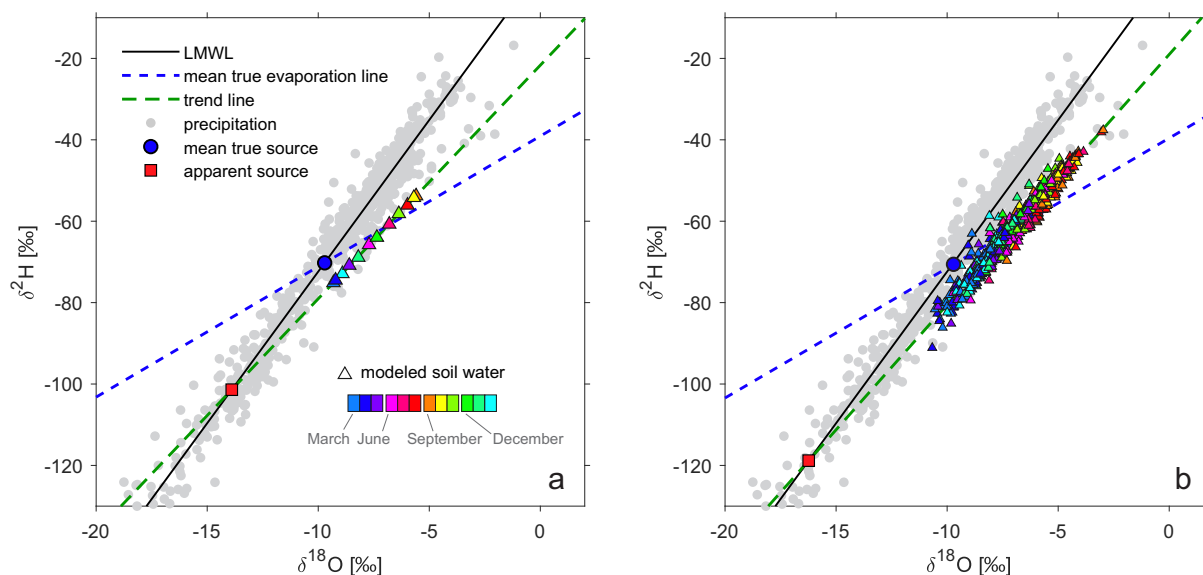
Figure 7. Isotopic composition of modeled soilwaters (triangles) obtained by mixing evaporated source waters through an exponential function. Soil water isotopic compositions are obtained starting from (a) long-term monthly sources (as in Figures 4-6), and (b) individual monthly isotopic sources, recorded at Vienna Hohe Warte station between 1961 and 2015 (grey dots).
