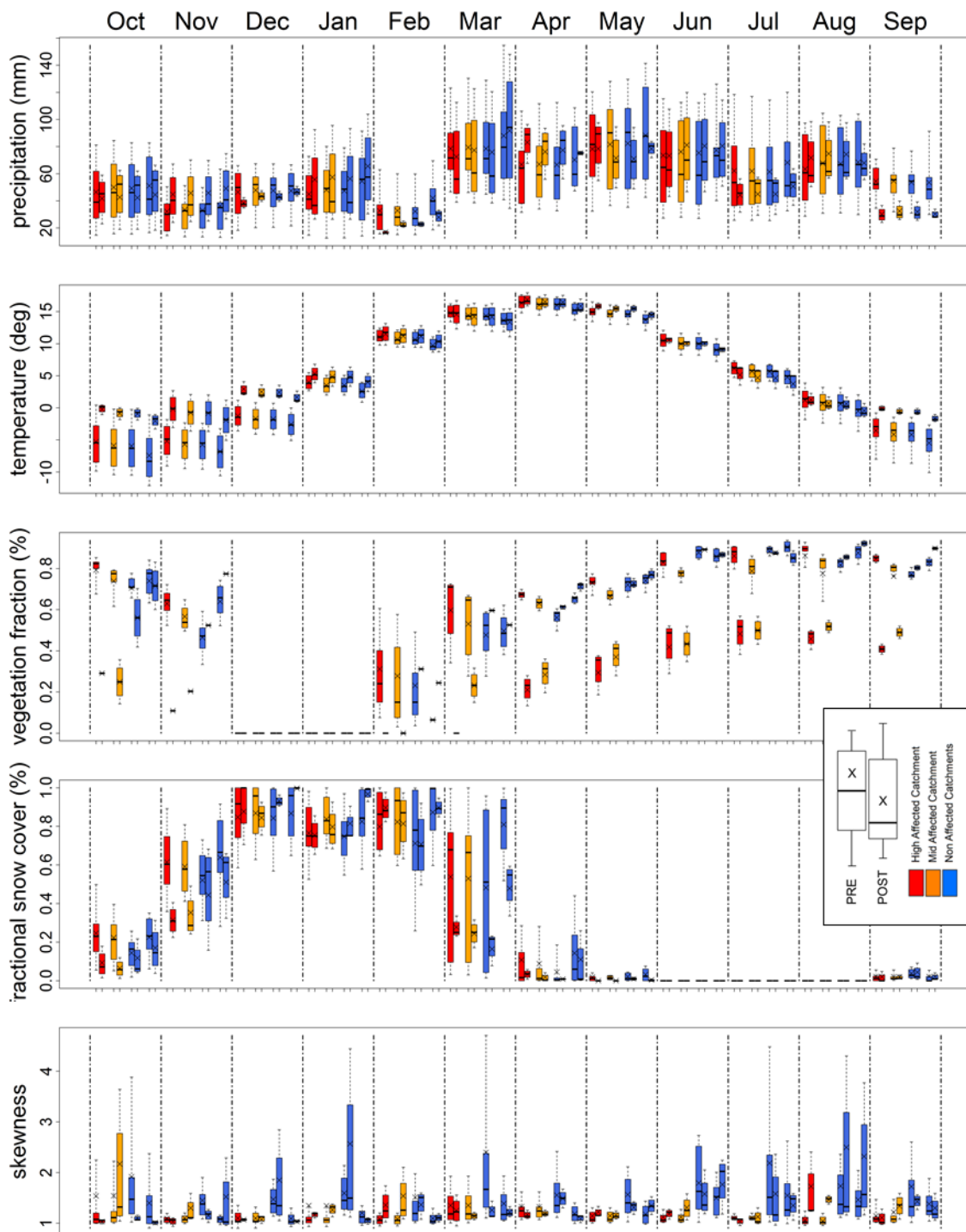
Figure A2 Seasonal distribution of the 13 descriptor defined at monthly scale for the pre- and post-wildfire period in each of the four selected sites. Red box high affected site; orange box mid affected site and blue boxes, non-affected areas.
