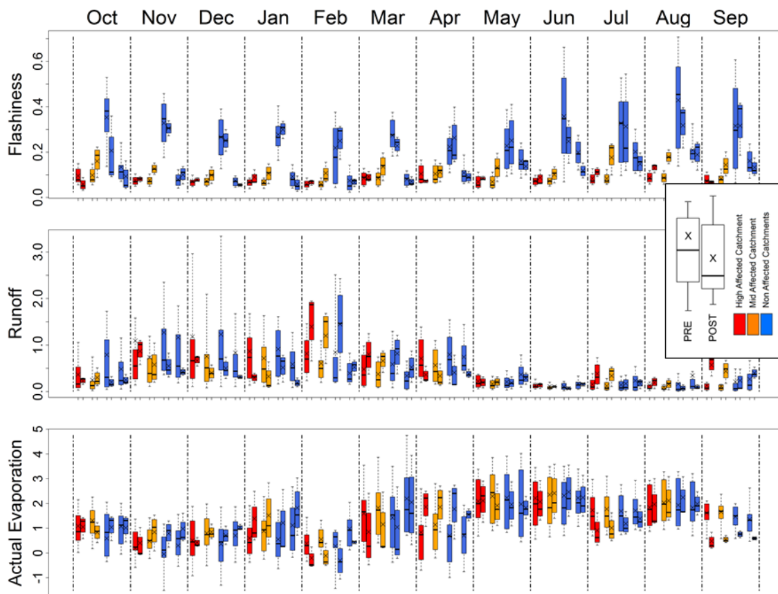
Figure A2 Seasonal distribution of the 13 descriptor defined at monthly scale for the pre- and post-wildfire period in each of the four selected sites. Red box high affected site; orange box mid affected site and blue boxes, non-affected areas (cont)
