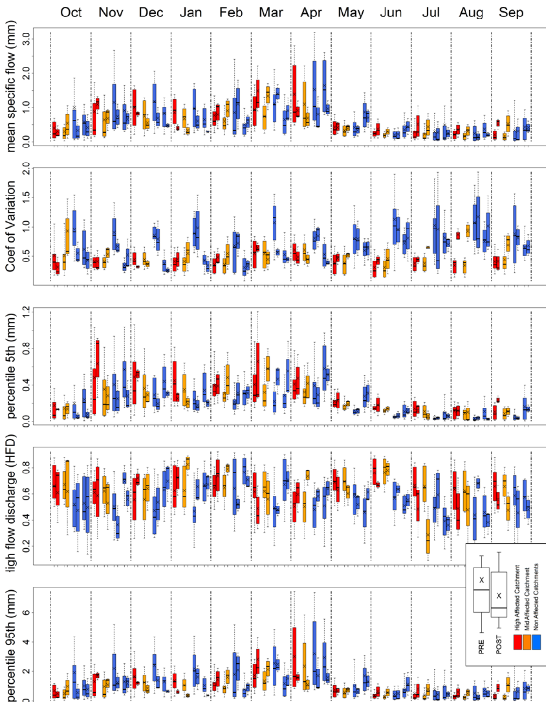
Figure A2 Seasonal distribution of the 13 descriptor defined at monthly scale for the pre- and post- wildfire period in each of the four selected sites. Red box high affected site; orange box mid affected site and blue boxes, non-affected areas (cont)
