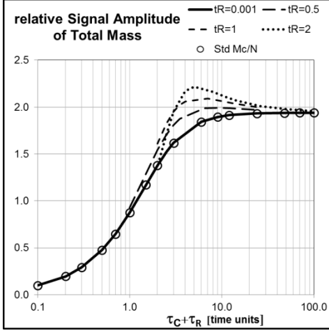
5 Fig.3: Signal Amplitudes of Total mass normalized by recharge: \sigma_{MT}/\sigma_N versus total mass time constant \tau_T = \tau_C + \tau_R for different river time constants \tau_R
