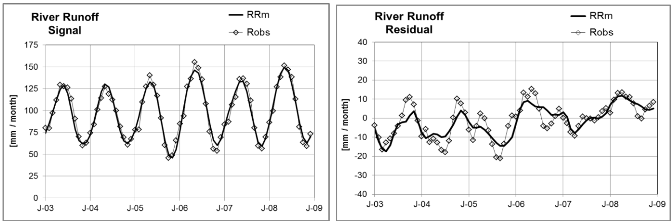
Fig.8: Time series of river runoff RR_m for the Amazon basin (Obidos) and optimization versus GRACE (a) for the signal (b) for the residual
