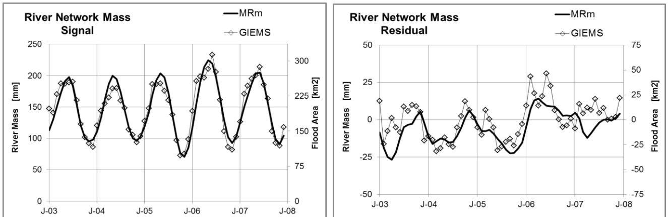
Fig.10: Time series of River network storage MR_m and inundated area from GIEMS for the Amazon (a) for the signal (b) for the residual
