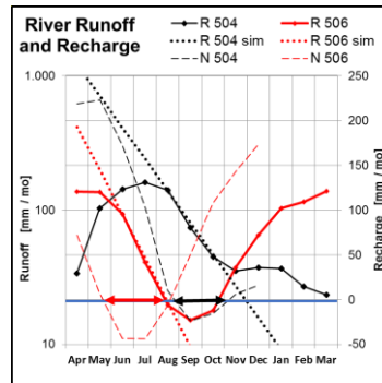
Fig.1d: Mean monthly Runoff R and Recharge N for seasonally dry catchments in the Amazon basin (Log scale for R) incl. exponential fittings for Runoff R_{sim}
