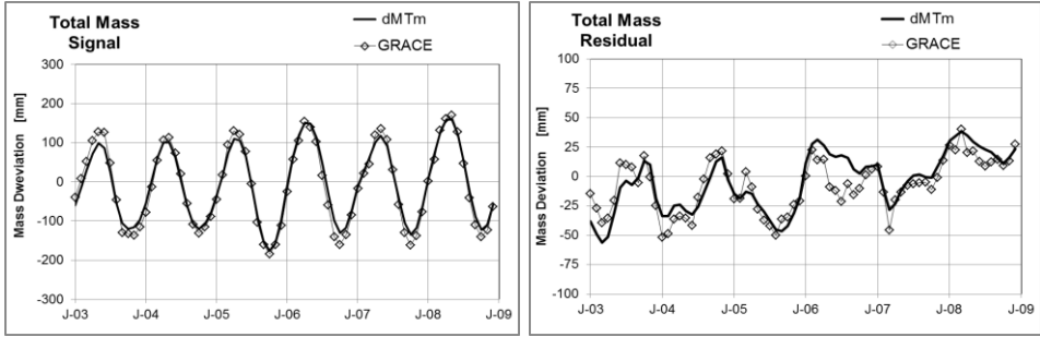
5 Fig.9: Time series of Total mass anomalies dM_T^I for the Amazon and optimization versus GRACE (a) for the signal (b) for the residual
