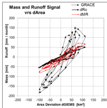
Fig.12: GRACE mass, calculated river network mass dM_R^R and observed river runoff dR_o versus Flood Area dGIEMS ; all displayed as anomalies (please consider dM_R^R = dR_o \cdot \tau_R^R = 1.53 \cdot dR_o )
