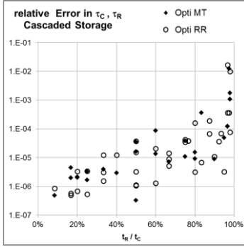
Fig.7: Relative error \varepsilon(\underline{\tau}_X)/\tau_X of the time constants \tau_C and \tau_R for the Cascaded Storage approach with respect to optimizations versus Total mass M_T^T or versus river runoff R_R^R .
