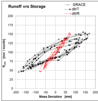
Fig.11: R-S relationships for observed runoff R_o versus the mass anomalies of GRACE, calculated Total mass dM_T^T and river network mass dM_R^R
