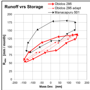
Fig.1a: R-S diagram with counter clockwise hysteresis for mean monthly observed runoff R_o versus GRACE dM for fully humid catchments incl. a phase adaption for Amazon upstream Obidos (Riegger and Tourian, 2014)
