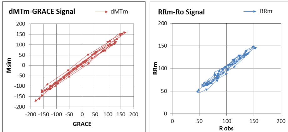
Calculated total drainable mass anomaly dM_T versus GRACE signal
