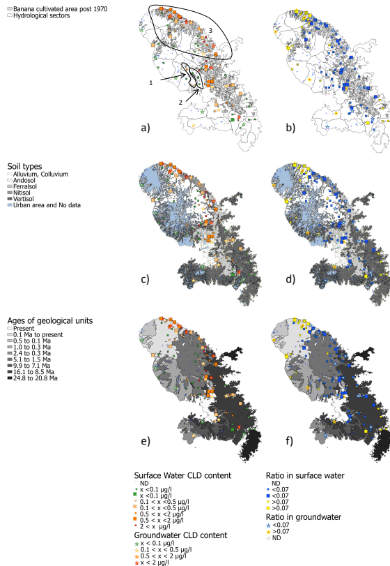
Fig. 2. Distribution of water CLD content (a, c, e) and 5bCLD / CLD ratio (b, d, f) for SW (square) and GW (star), according to banana cultivated areas and hydrological sectors (a and b), soils (c and d) adap
