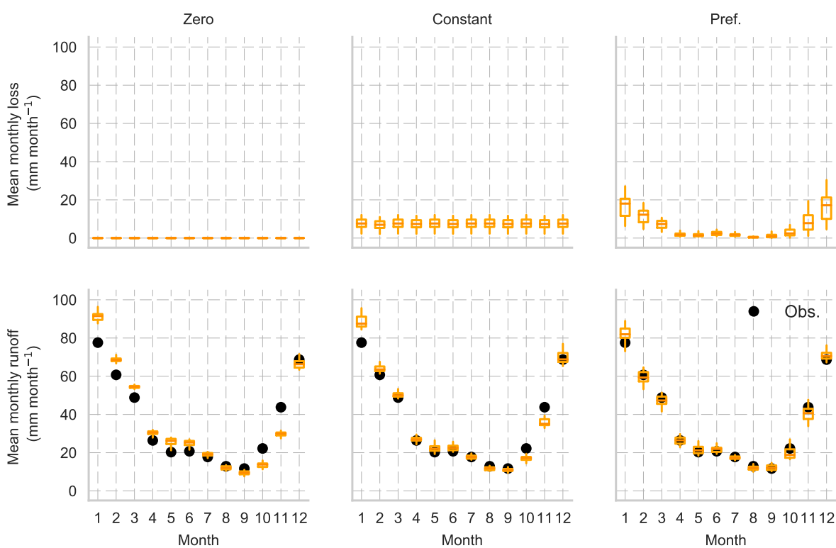
Figure 8. Upper row: mean monthly loss between 2007-2016 for the feasible model realizations in the Semois catchment at Sainte-Marie. Lower row: mean monthly discharge between 2007-2016 for the feasible model realizations (orange) and observations (black dots) for the three models at Sainte-Marie. The preferential model leads to better performances with lower simulated runoff in the first half year and higher runoff in the wetting up period (Oct-Nov).
