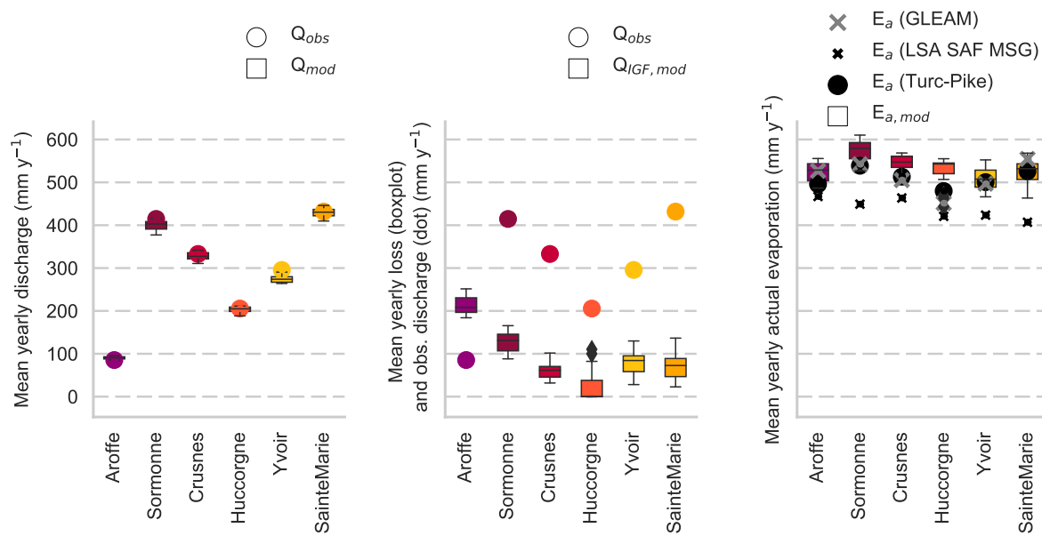
Figure 12. Water balance components of additional modeled catchments over the period 2007-2016. Left: modeled (boxplot) and observed (dot) mean yearly discharge overlap well. Middle: modeled mean annual net loss (boxplot) and observed mean yearly discharge (dot), showing the large proportion of net intercatchment groundwater flows especially in the Aroffe catchment. Right: modeled actual evaporation (boxplot), GLEAM actual evaporation (grey cross), LSA SAF actual evaporation (black cross) and Turc-Pike estimates (black dot). It should be noted that LSA SAF estimates are only available during the validation period (2012-2016). Model results overlap relatively well with GLEAM and Turc Pike estimates of actual evaporation, but LSA SAF estimates are lower.
