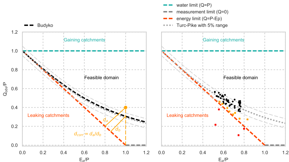
Figure 3. Left: Dimensionless representation of the runoff coefficient ( Q_{obs}/P ) as a function of the dryness index ( E_p/P ), referred to as the Budyko framework. The red line is the energy limit ( Q_{obs} = P - E_p ) beyond which catchments are leaking water; the blue line is the water limit ( Q = P ) above which catchments are gaining water; the dark grey line is the measurement limit ( Q = 0 ). The domain within these three limits is the theoretical feasible domain. The Turc-Pike and the Budyko curves plot very close to each other. The 5% uncertainty bound around the Turc-Pike curve is also shown. For each catchment, the ratio of the distance to the energy limit ( d_a ) over the distance of Turc-Pike to the energy limit ( d_b ) is used as a proxy for the presence of net intercatchment groundwater flows. Right: the catchments of the Meuse basin are located around the Turc-Pike line (black circles). However, four catchments plot beyond the energy limit (red squares) and eight catchments plot very close to the energy limit and are beyond the lower 5% range of Turc-Pike (orange squares). In these catchments, we expect net intercatchment groundwater flow losses to occur.
