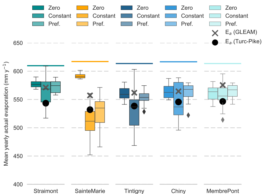
Figure 10. Best realizations of modeled mean annual actual evaporation in all stations in the Semois catchment for the three models during 2007-2016 (boxplots show from left to right: zero, constant and preferential model results). Colored horizontal lines indicate mean annual potential evaporation used as forcing. Estimates of actual evaporation from the Turc-Pike line are shown as black dots and GLEAM estimates are shown as grey crosses. In the catchment of Sainte-Marie, the reference model without net intercachment groundwater flows overestimates actual evaporation compared to the other two models and Turc-Pike estimates.
