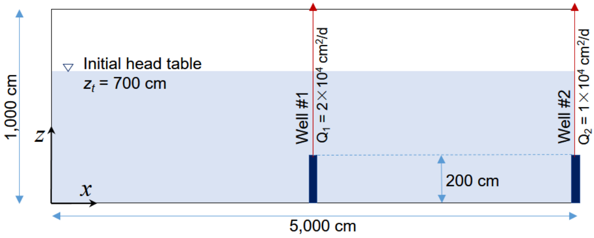
Figure 4: Schematic of the cross-sectional for test case 2. Two pumping wells with screens of z = 0 - 200 cm are located at x = 2,500 cm and 5,000 cm. The pumping rates per unit width at well #1 and #2 are respectively 2 \times 10^4 \text{cm}^2/\text{d} and 1 \times 10^4 \text{cm}^2/\text{d} , respectively.
