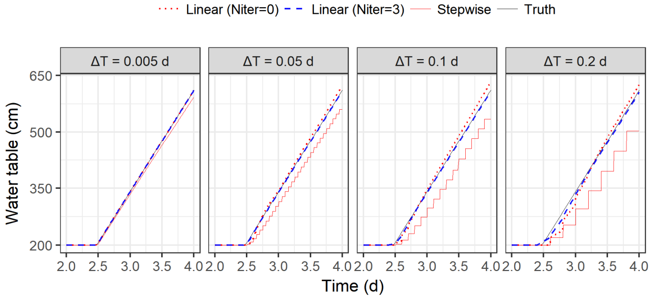
Figure 9: Water table changing with time for different macro time step sizes ( \Delta T = 0.005 d, 0.05 d, 0.1 d, and 0.2 d), in scenario 1, case 1. The HYDRUS1D solution is taken as the “truth”. Compared with the stepwise extended method (Seo et al., 2007), the coupling error is significantly reduced by a linear prediction.
