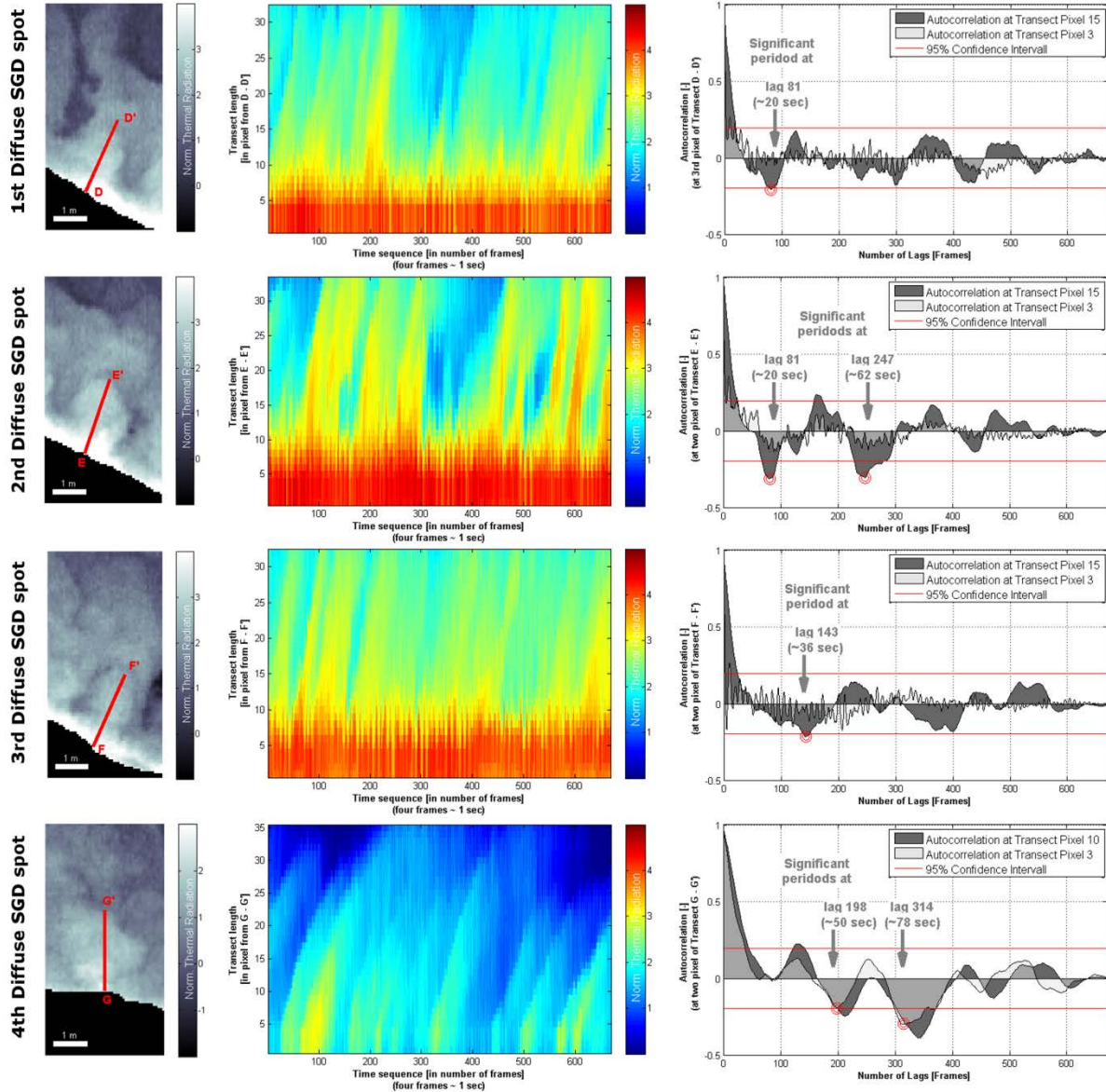
Figure 6: Analyses of spatiotemporal behavior and potential periodicity of diffuse SGD spots are presented. Spot locations are outlined in Fig. 1 and Fig.3 indicated by the location of the counter rotating vortex pairs (CVP). The first column shows transects across the maximum extent and midpoint position of diffuse SGD spots (note that the spatial scale varies between each spot indicated through the scale bar at the lower left of each subset). The middle column shows the normalized thermal radiance (NTR) values along transects over time. The third column shows the temporal autocorrelation of NTR values along the entire time series obtained at the midpoint of the transect. Those points reflect the most unaltered discharge signals (the larger value). As reference, we show the third transect pixel (close to the shoreline) as well in order to outline the wave influence on the periodicity.
