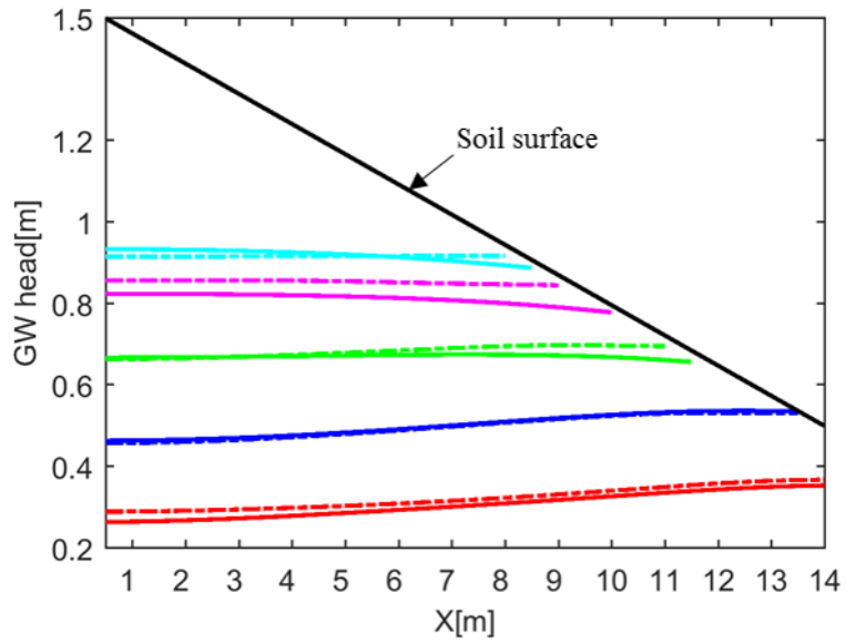
Figure 78. Simulated water table level after 4 (red), 8 (blue), 12 (green), 16 (magenta) and 20 days (sky blue) with MIKE_SHE (solid lines) and MOBIDIC-MODFLOW (dashed lines).
