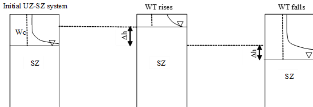
Figure 56. Conceptualization of the interaction between UZ-SZ in MOBIDIC-MODFLOW in rising and falling water table conditions.
