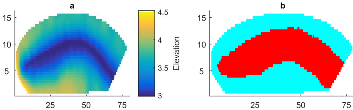
5 Figure 89. a) The digital elevation model of Borden catchment and b) zoning map of the catchment based on depth to water table less than 1.5m (red) and greater than 1.5m (blue).
