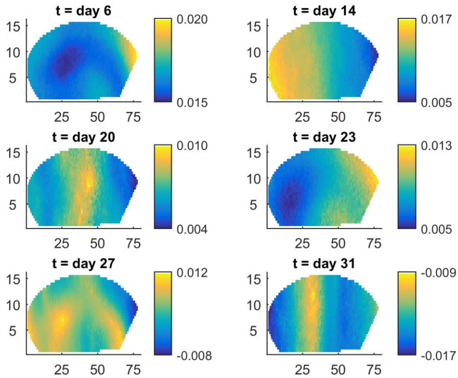
Figure 9.10. The difference in simulated water tables by MIKE_SHE and MOBIDIC-MODFLOW ( h_{MOBIDIC} - h_{MIKESHE} ) [m] at different time steps.
