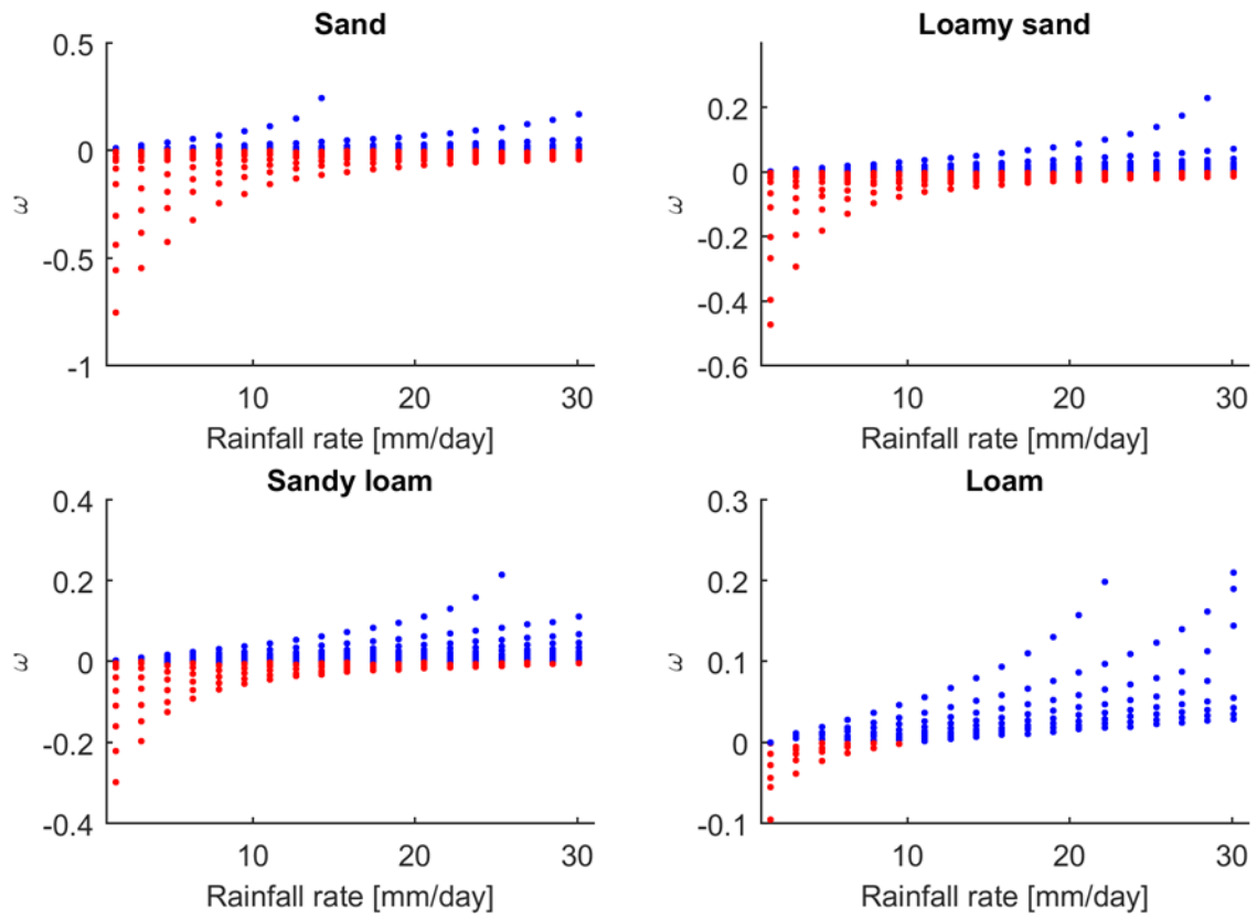
Figure 67. Variations in \omega against rainfall intensity for different initial water table level and soil types.
