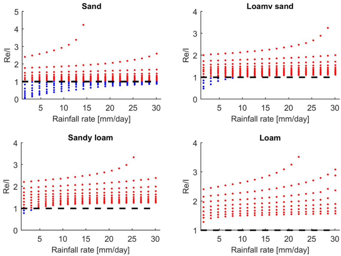
Figure 45. Variations of the ratio of recharge/infiltration with rainfall and initial depth to water table in different soil types simulated by MIKE_SHE. The red dots are \frac{Re}{I} \geq 1 and the blue dots are \frac{Re}{I} < 1 .
