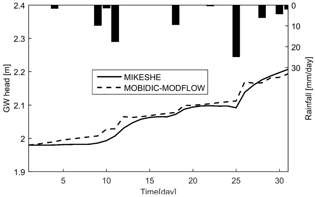
Figure 10.11. Simulated water table depth by MIKE SHE (solid lines) and MOBIDIC-MODFLOW (dashed lines) at the outlet grid of Borden catchment.
