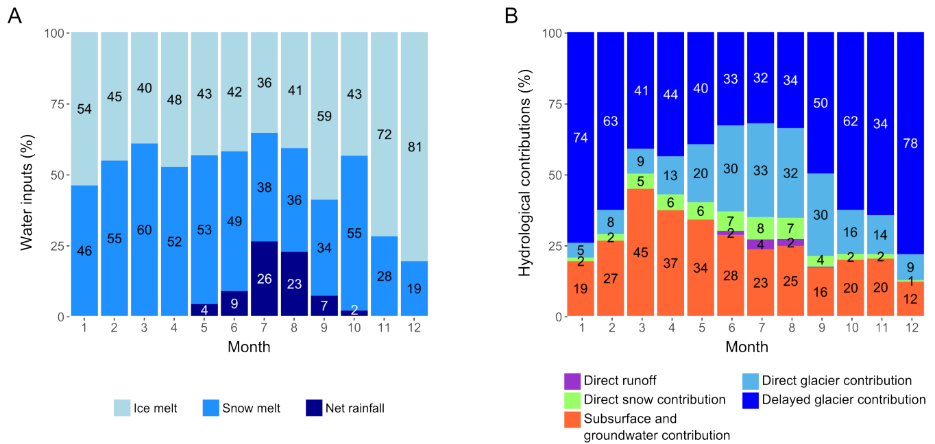
Figure 14. Average monthly contributions to the water input (definition 1, ch. 3.2.5) (a) and hydrological contributions (definition 2, ch. 3.2.5) (b) simulated with configuration v3 for the years 2012-2015.
