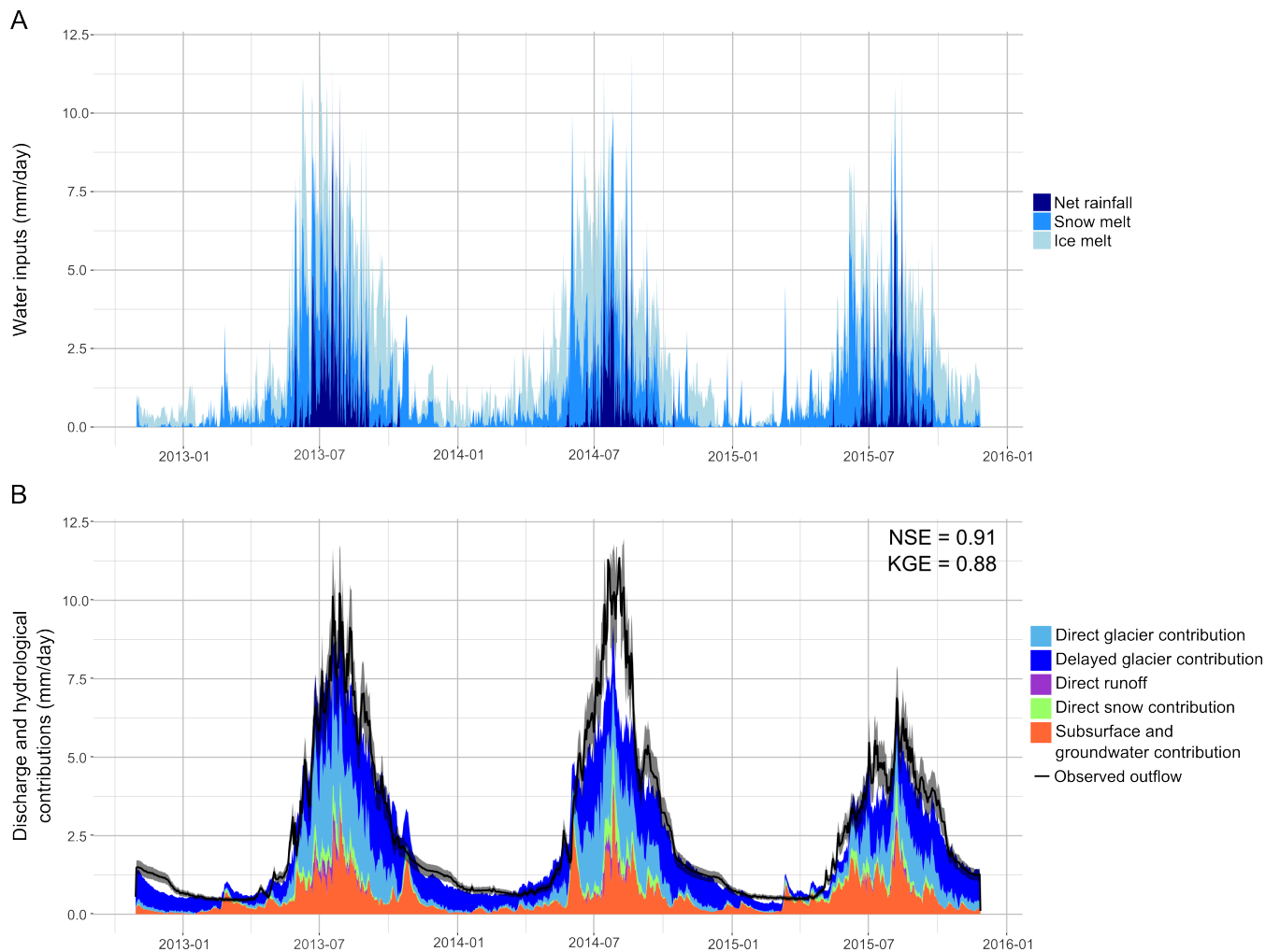
Figure 13. Daily discharges and flow components simulated with configuration v3: (a) production of ice melt, snow melt and net rainfall (note that the sum of the flow components represent the total water input and is not equal to the discharge at the catchment outlet, see definition 1, ch. 3.2.5) (b) hydrological contributions to the outflow (definition 2, ch. 3.2.5). Observed discharges are represented by the black line with a 15 % interval of error.
