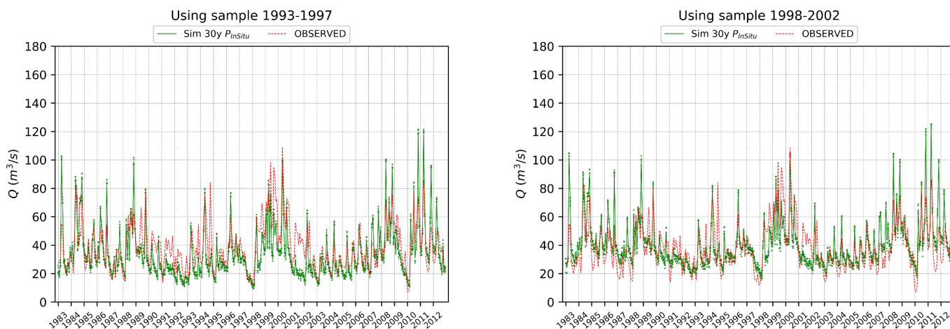
Figure 3. Observed and simulated discharge for the Coello River at Payende with 30 years (1983-2012) of In-Situ precipitation (Sim 30y P_{in-Situ} ) for calibration samples 1993-1997 and 1998-2002, with the sample used to calibrate the model indicated in the header.
