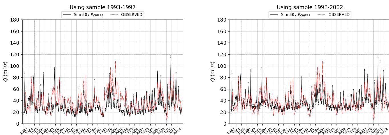
Figure 4. Observed and simulated discharge for the Coello River at Payende with 30 years (1983-2012) of CHIRPS precipitation (Sim 30y P_{CHIRPS} ) for calibration samples 1993-1997 and 1998-2002, with the sample used to calibrate the model indicated in the header.
