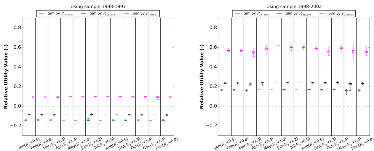
Figure 13. Relative Utility Value using simulated river discharge of 5 years for water scarcity happening independently in any one month. K_y is the sensitivity of the crop to water deficit. Boxplots show the median, interquartile range and minimum-maximum range.
