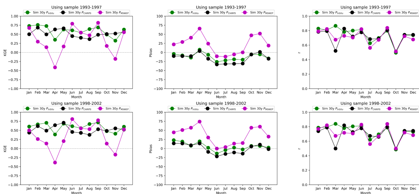
Figure 6. KGE, Pbias and r performance metric for simulated river discharge for the complete time period of 30 years (1983-2012) using three different precipitation datasets (In-Situ, CHIRPS and MSWEP) in the Coello basin. Two calibration samples are shown (1993-1997, 1998-2002), with the sample used to calibrate the model indicated in the header.
