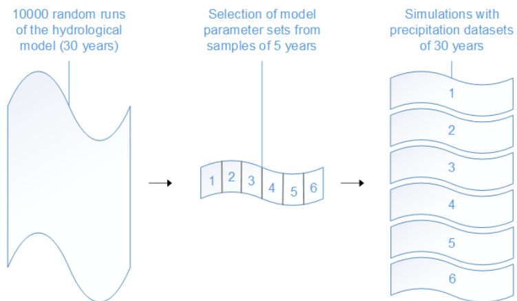
Figure 2. Obtaining hydrological model simulations from the six samples of 5 years of observed river discharge.
