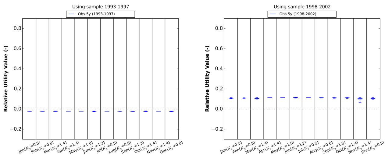
Figure 11. Relative Utility Value using observed river discharge of 5 years for water scarcity happening independently in any one month. K_y is the sensitivity of the crop to water deficit. Boxplots show the median, interquartile range and minimum-maximum range.
