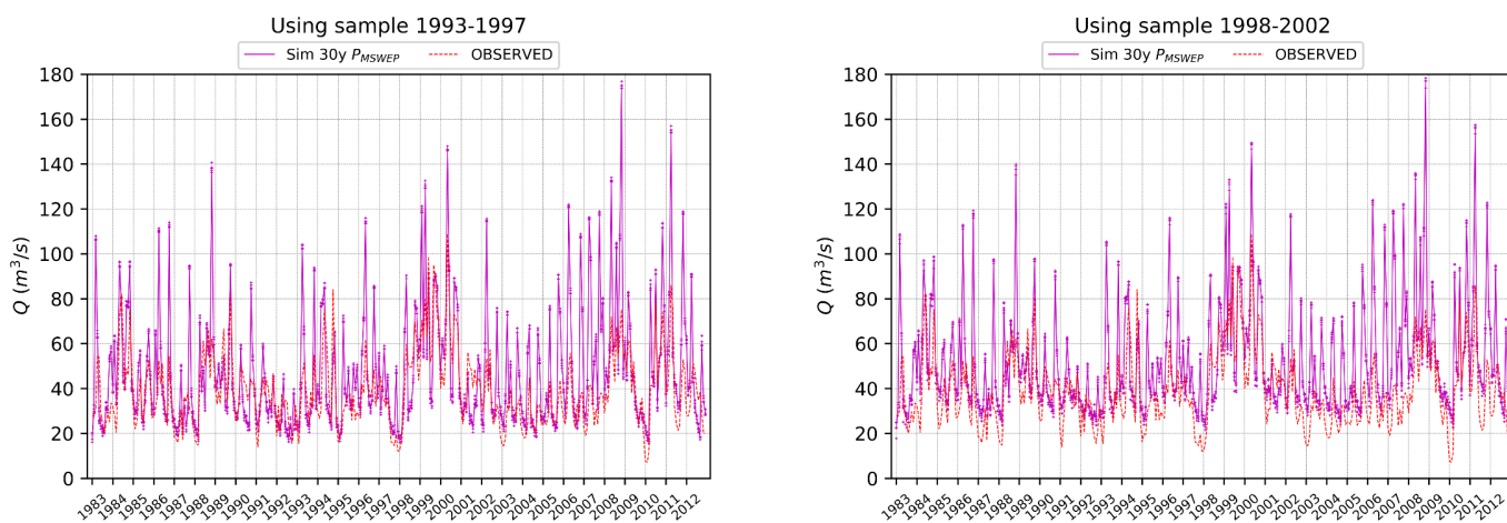
Figure 5. Observed and simulated discharge for the Coello River at Payende with 30 years (1983-2012) of MSWEP precipitation (Sim 30y P_{MSWEP} ) for calibration samples 1993-1997 and 1998-2002, with the sample used to calibrate the model indicated in the header.
