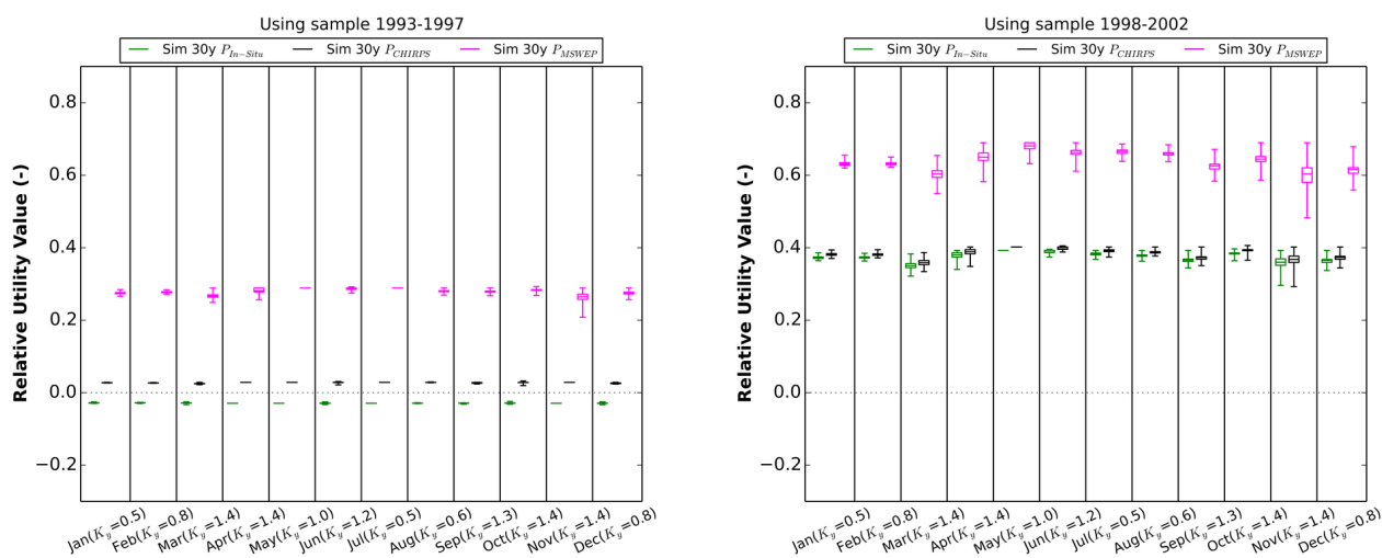
Figure 12. Relative Utility Value using simulated river discharge of 30 years for water scarcity happening independently in any one month. K_y is the sensitivity of the crop to water deficit. Boxplots show the median, interquartile range and minimum-maximum range.
