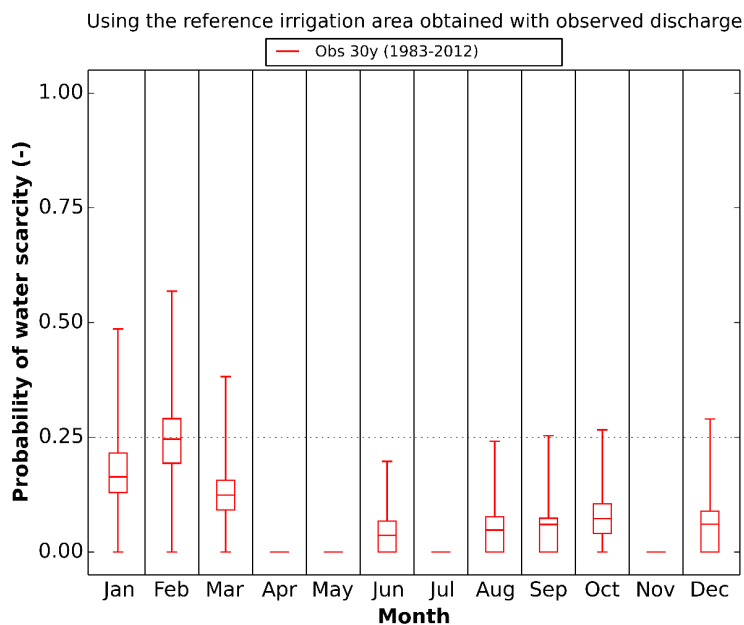
Figure 7. Probability of water scarcity using the reference irrigation area obtained with the observed river discharge of 30 years (Obs 30y) and the reference surface water availability. Boxplots show the median, interquartile range and minimum-maximum range.
