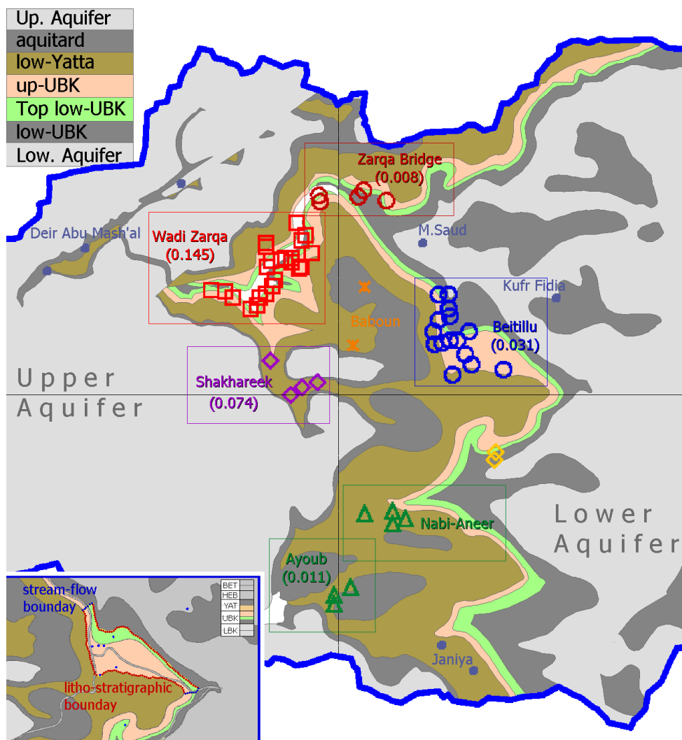
Figure 6: Spring groups in Wadi Natuf Note: Six spring groups were identified in central Natuf, with two in the North (Zarqa), two in the centre (Beitillu & Shakhareek) and two in the South ('Ayoub & Nabi Aneer). The recharge areas of these perched intermediate aquifers are isolated by outcropping bottom aquicludes (Figures 2a, b and 3a). Source: geological map based on GSI, 2000, 2008
