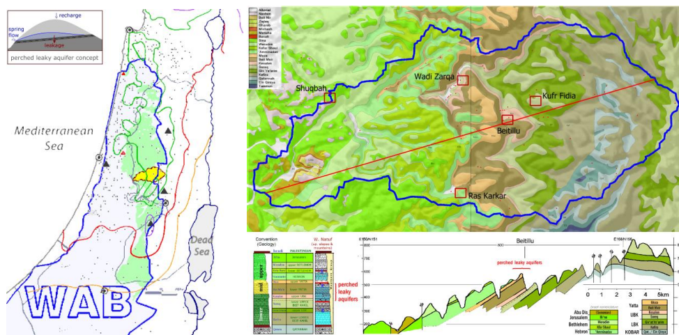
780 Figure 1.a. Left – Location map and concept inlet; Wadi Natuf (yellow) positioned in the mountains and slopes of the WAB; WAB boundary, aquifer outcrop area (green), isohyets, rainfall stations, main weather stations, main spring outlets (modified after Ettinger, 1996) and schematic concept of perched, leaky aquifers; Figure 1.b. Right – Geological relief map, cross-section, main springs and soil moisture locations (red boxes) (Sources: geological map modified after GSI, 2000, 2008; stratigraphic column modified after (Dafny et al. 2010).
