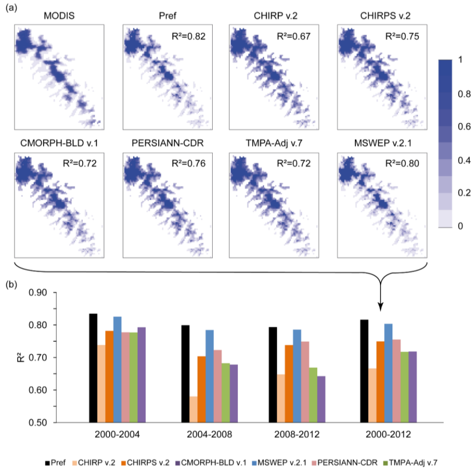
5 Figure 8: Observed (gap-filled MODIS snow-products) versus simulated snow cover duration (SCD) using P_{ref} and SPPs as input data in the snow model: (a) Maps of snow cover duration for 2000–2012; (b) Efficiency ( R^2 scores) of simulated SCD versus MODIS SCD for the different calibration periods. SCD are expressed as the percentage of days over the simulation period. R^2 values stand for the grid-cell-to-grid-cell correlation between the observed and simulated SCD. Green and red stars highlight SPPs with closest and further precipitation estimates to P_{ref} over the subset considered.
