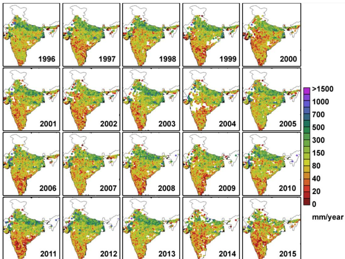
Figure 4: Maps showing gridded ( 0.1^{\circ} \times 0.1^{\circ} ) groundwater recharge (mm/yr) calculated using WTF method. Blank area represent areas of no data availability.
