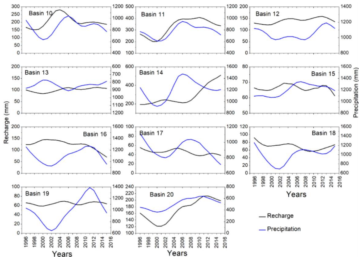
Figure 7: Basin-wide estimates of Hodrick-Presscott trend analysis of R_g (mm/yr) and precipitation (mm/yr). For basin locations, see Figure 1.
