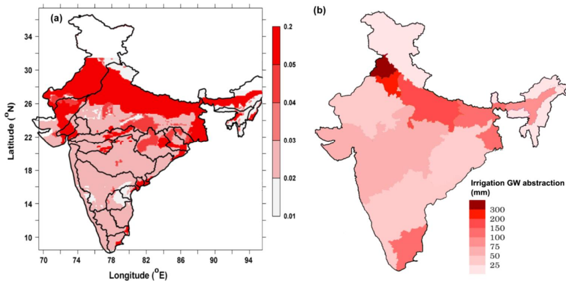
Figure 3: Maps of (a) specific yield data (modified from Bhanja et al. , 2016). Blank area represent areas of no data availability; (b) state-wise groundwater abstraction for irrigation (mm, estimates are for the year 2009) (CGWB, 2012a).
