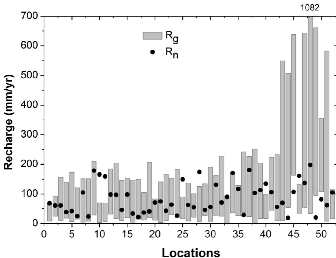
Figure 9: Comparison of groundwater recharge rates obtained from the present study (annual range) and some of the earlier studies conducted over the point locations shown in Figure 1. Recharge estimates exceeded 700 mm/yr data were indicated on the top of the column.
