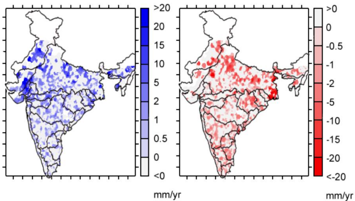
Figure 6: Maps of positive and negative trends in groundwater recharge in 1996-2015. Basin boundaries are overlaid. Blank area represent areas of no data availability.
