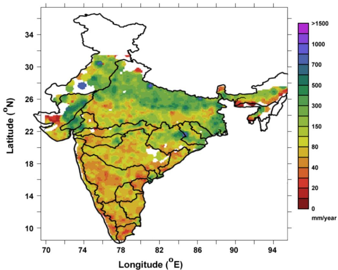
Figure 5: Map of mean recharge in the study period (1996-2015). Blank area represent areas of no data availability.
