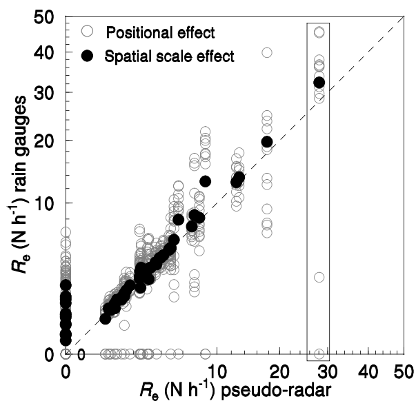
10 Figure 6: Event erosivity R_e at 12 rain gauges located within a 1 \text{ km}^2 pixel versus R_e based on pseudo-radar data calculated from the hyetographs of the 12 rain gauges (open grey circles). Filled black circles show the average R_e of all 12 rain gauges vs the R_e from pseudo-radar rainfall. Note that the average R_e can be considerably larger than zero while the averaged rainfall of the pseudo-radar remains below the thresholds of erosivity (black circles along the y axis). Rectangular frame shows variation of R_e for a single day. Axes are square-root scaled to improve resolution at low R_e .
