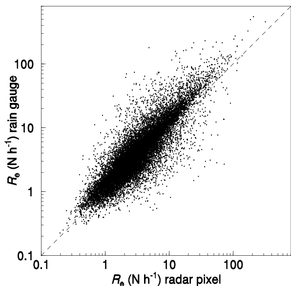
5 Figure 5: Comparison of event erosivity R_e calculated from radar data and R_e from rain gauge data for 115 radar pixels that enclose a rain gauge. Only events that were erosive at both scales (19 944 events) during the 16 year period are shown. The dashed line represents unity. Axes are log scaled. Note: no spatial scaling factor or method factor was applied because these factors also included the effect of incomplete coverage of the pixel by an erosive rain cell.
