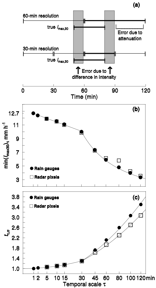
Figure 2: a) Time periods influencing the underestimation of I_{\max30} when temporal resolution is 30 min (or more) or when temporal resolution is 60 min (or any resolution >30 min). b) Minimum threshold for I_{\max30} ( \min(I_{\max30})_{\tau} ) derived from rain gauge (solid circles) and radar data (open squares) required to obtain the same number of erosive events as with a temporal resolution of 1 min; lines show Eq. (6.1) and Eq. (6.2) (RMSE is 0.10 and 0.39). c) Scaling factor t_{\tau,\sigma} to scale R_c or R for temporal resolution \tau when spatial resolution \sigma is either rain gauge scale (solid circles) or 1 x 1 km 2 (open squares) respectively; lines show Eqs. (7.1), (7.2) and (7.3) (for all RMSE \leq 0.04 ). The x-axes in b) and c) are square-root scaled.
