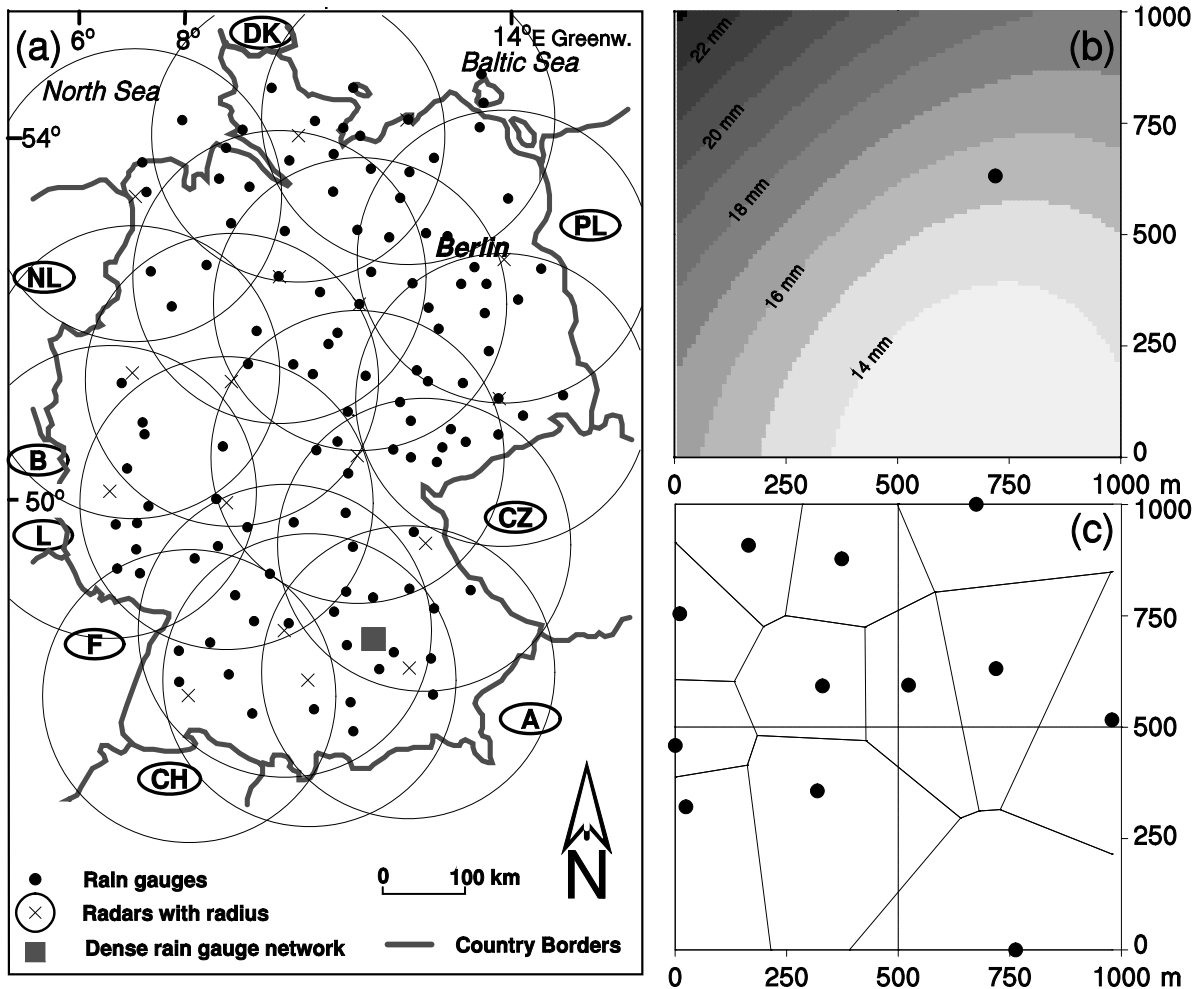
10 Figure 1: a) Locations of the 115 rain gauges (dots), the coverage (circles) of the 17 weather radars (crosses) and the location of the 12 rain gauges used for the pseudo-radar data (square; size exaggerated) in Germany. b) One rain gauge (dot) within one 1 x 1 km 2 pixel (bounding box) and isolines of rain depth (taken from Fiener and Auerswald, 2009) illustrating the variability of a single erosive rain event at 1 x 1 km 2 grid scale causing positional effects. c) Distribution of the 12 rain gauges (dots) within an area of 1 x 1 km 2 (bounding box) and their corresponding Thiessen polygons. Dashed lines separate the area to a spatial scale of 0.5 x 0.5 km 2 .
