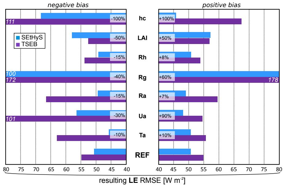
Figure 5. Sensitivity analysis to positive and negative realistic biases applied to meteorological and vegetation inputs for both models.
