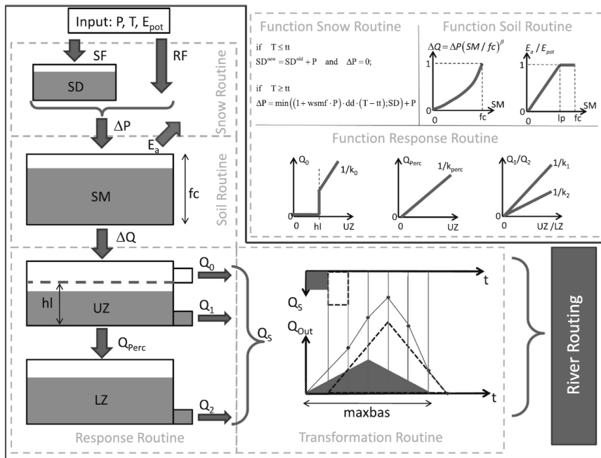
15 Figure 3: Vertical structure of the HBV-IWW model according to Wallner et al. (2013)
