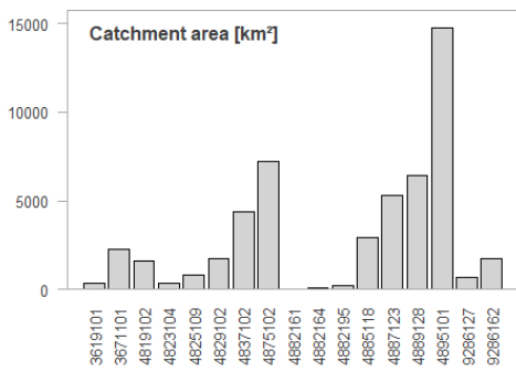
Figure 12: Catchment areas of the considered gauges.
