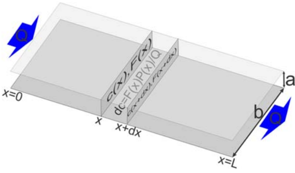
Figure 2: Discretization and mass conservation in a basic network element; a 1D fracture. The conservation of mass requires that the change of concentration between x and x+dx is proportional to the surface of a section P(x)dx , where P(x) is a perimeter, to the dissolution rates F(x) , and inversely proportional to the flow rate Q .
