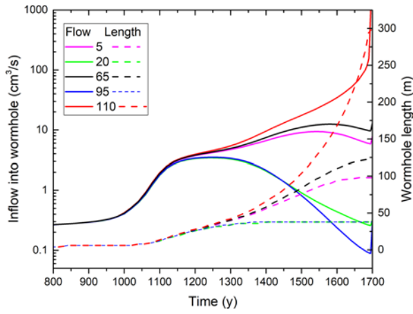
Figure 16: Evolution of input flow rates (solid lines) and wormhole lengths (dashed lines) for the wormholes marked in Fig. 15.
