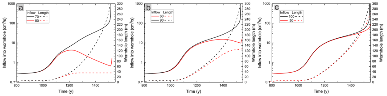
Figure 14: Temporal evolution of flow (full lines) and length (dashed lines) of the interacting wormholes of Figure 12. Lettering Labels corresponds to Figure 12.
