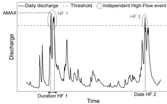
Figure 1: Selection and characterisation in terms of frequency, magnitude, duration, and time of year of: (a) Floods (HF: High-Flow event, AMAX: Annual Maximum POT), and (b) Droughts (LF: Low-Flow event).
