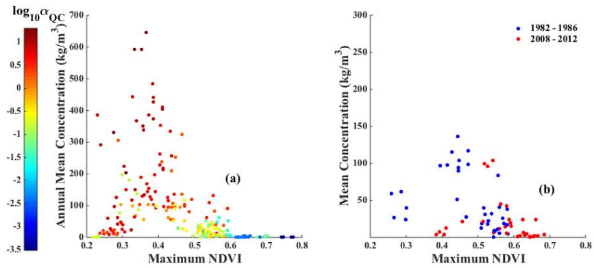
Fig. 2. Figure 3R1: Scatter plot of annual mean concentration and maximum NDVI: (a) at 44 study gauges between 1982 and 1986, where the dots are color-coded by the slope in the Q-C regression ( \log_{10} \alpha_{QC} ) at each ga
