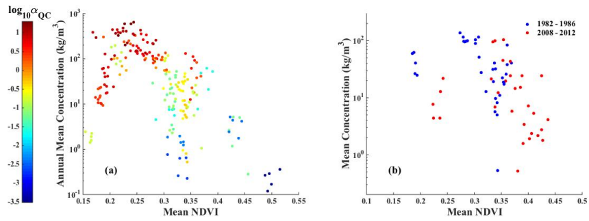
Fig. 6. Figure 3R4: Scatter plot of annual mean concentration and mean NDVI: (a) at 44 study gauges between 1982 and 1986, where the dots are color-coded by the slope in the Q-C regression ( \log_{10} \alpha_{QC} ) at each gauge
