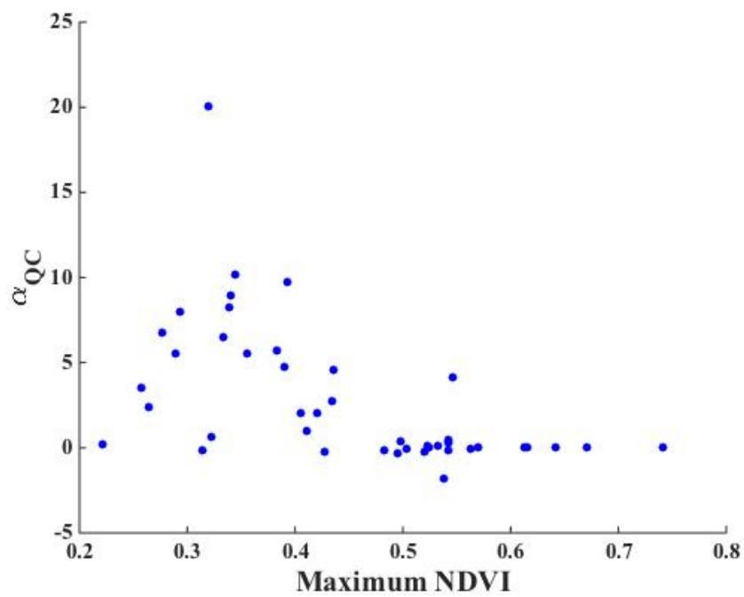
Fig. 1. Figure 2R1: Scatter plots between the maximum NDVI and slope in the Q-C regression ( \alpha_{QC} ).
