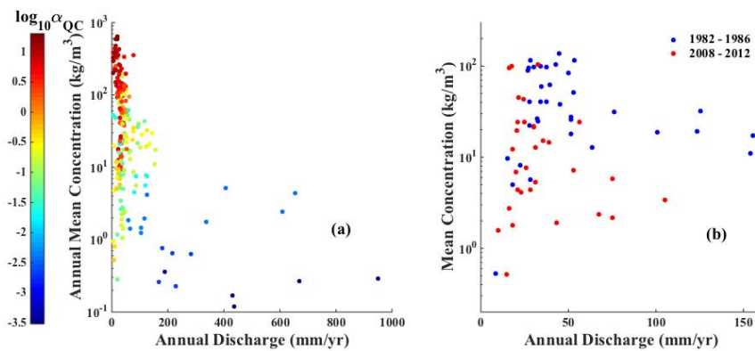
Fig. 5. Figure 3R3: Scatter plot of annual mean concentration and annual discharge: (a) at 44 study gauges between 1982 and 1986, where the dots are color-coded by the slope in the Q-C regression ( \log_{10} \alpha_{QC} ) at each
