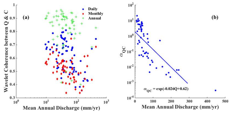
Fig. 8. Figure 1: Scatter plots between long-term mean annual discharge ( Q_m ) and (a) wavelet Q-C coherence at daily, monthly and annual scales, (b) slope of the discharge- sediment concentration regression ( \alpha_{QC} )
