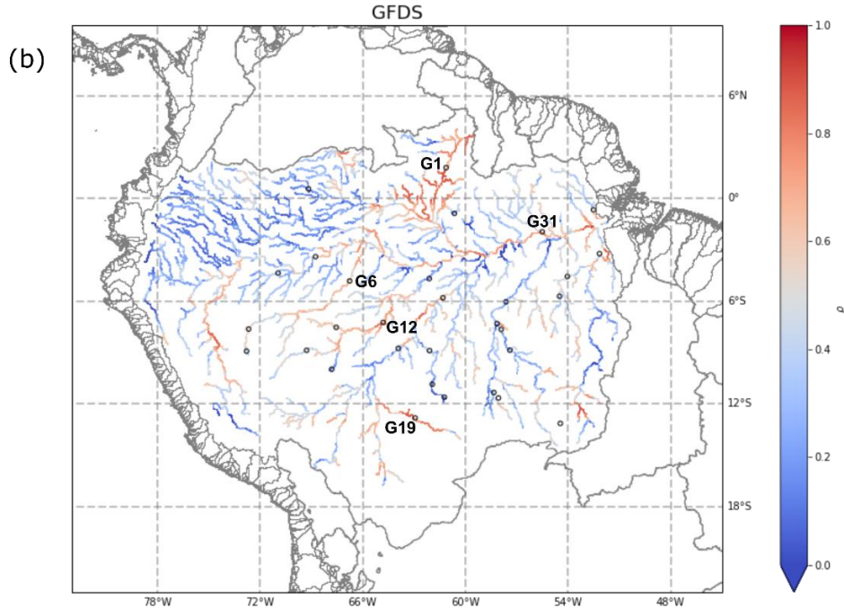
Figure 4 Spearman correlation ( \rho ) between modelled river channel storage and MODIS (a) and GFDS (b) water extent using the Optimal Grid Cell Selection method (Method A) with a search window of 0.55^\circ \times 0.55^\circ (circle: gauging station; circle with black label: potential SGRs sites where gauging data is available). (continued)
