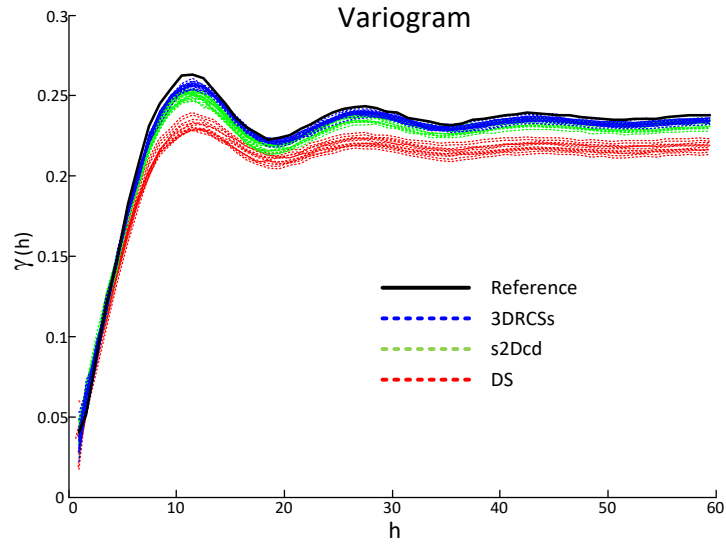
Figure 11. Comparison of the variograms between DS, s2Dcd and 3DRCSs.
