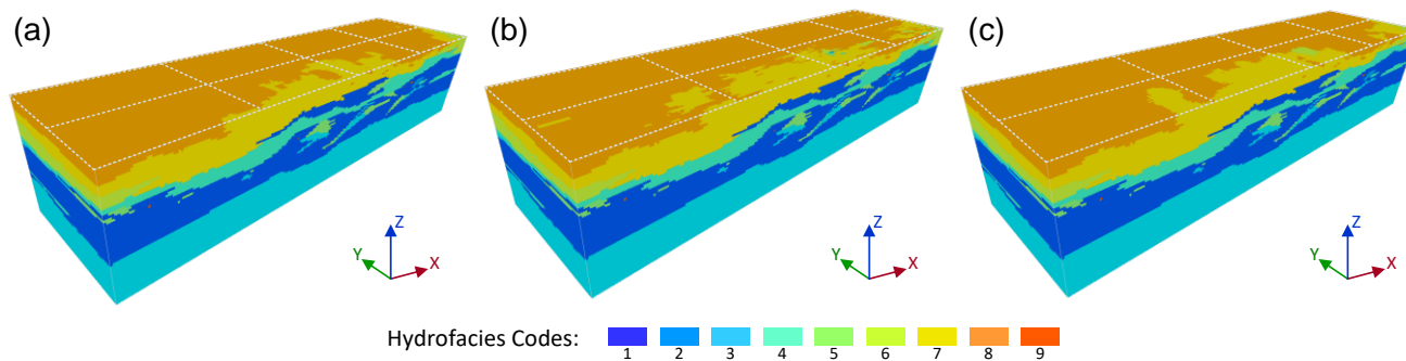
Figure 16. Three realizations using three different MPS approaches: (a) DS, (b) s2Dcd with the coordinate z as auxiliary variable; and (c) 3DRCSs with the coordinate z as auxiliary variable.
