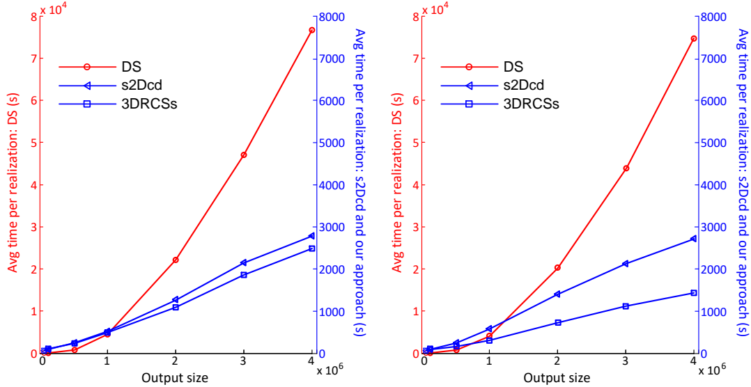
Figure 14. Comparison of computational performance between DS, s2Dcd and 3DRCSs with increasing the size of output grid: (left) two cross-sections and (right) four cross-sections in each direction. Note that different time axes are used in the two subplots, and four processors are used for DS-based reconstruction and s2Dcd but only one for 3DRCSs.
