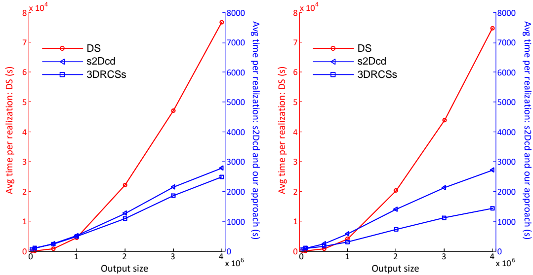
Figure 14. Comparison of computational performance between DS, s2Dcd and 3DRCSs our approach with increasing the size of output grid: (left) two cross-sections and (right) four cross-sections in each direction. Note that different time axes are used in the two subplots, and four processors are used for DS-based reconstruction and s2Dcd but only one for 3DRCSs our method .
