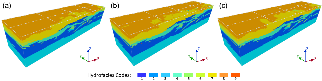
Figure 16. Three realizations using three different MPS approaches: (a) DS, (b) s2Dcd with the coordinate z as auxiliary variable; and (c) 3DRCSour approach with the coordinate z as auxiliary variable.
