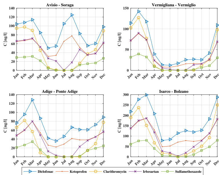
Figure 6. Monthly flux concentrations of 5 PPCPs (diclofenac, ketoprofen, clarithromycin, irbesartan and sulfamethoxazole) at the control sections of Soraga in the Avisio river, Vermiglio in the Vermigliana creek, Ponte Adige in the Adige river and Bolzano in the Isarco river. Concentrations are expressed in ng/l .
