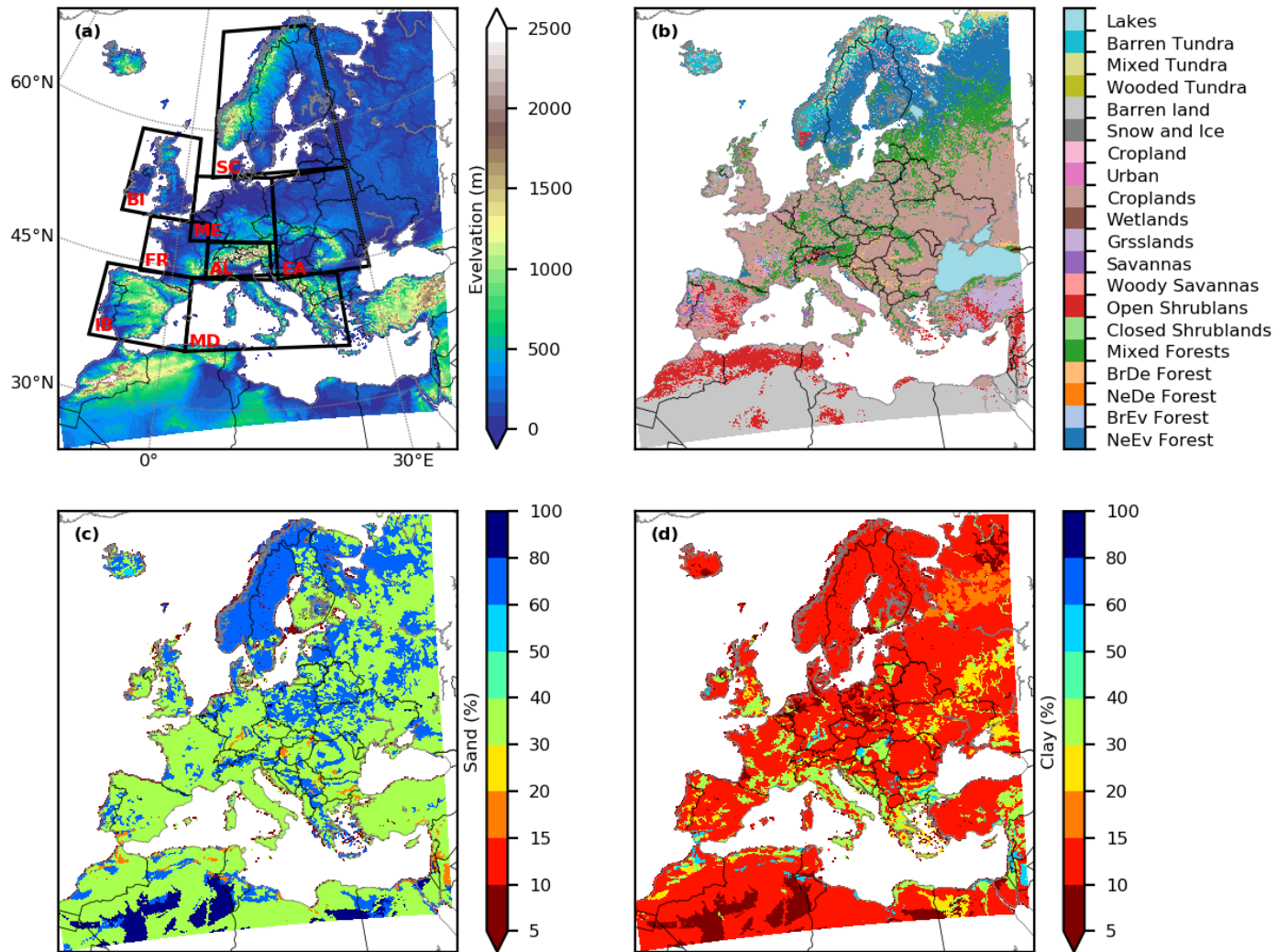
5 Figure 1. Model surface input data: a) USGS GMTED2010 DEM, b) dominant land use type based on MODIS data, c) percent sand content, and d) percent clay content based on global FAO soil database. The inner boxes in (a) show the boundaries of the PRUDENCE regions (FR: France, ME: mid-Europe, SC: Scandinavia, EA: Eastern Europe, MD: Mediterranean, IP: Iberian Peninsula, BI: British Islands, AL: Alpine region; Christensen and Christensen et al. , 2007).
