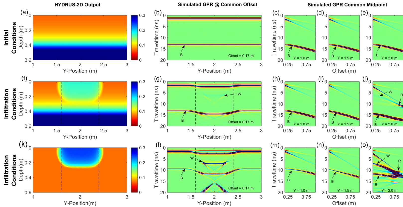
321 Figure 2: Panels (a), (f), and (k) show volumetric moisture distribution from HYDRUS-2D simulations used to generate simulated common-offset GPR data (b, g, 322 l) and multi-offset GPR data (c-e, h-j, and m-o). Vertical dashed lines indicate the extent of the wetted surface. Annotated arrivals are the bottom of sand layer 323 reflection (B), wetting front reflection (W), and refraction (R). Note that the base of sand reflection (B) is caused by the boundary at 0.60 m depth between the sand 324 and gravel, not the capillary rise shown in panels (a) and (f).
