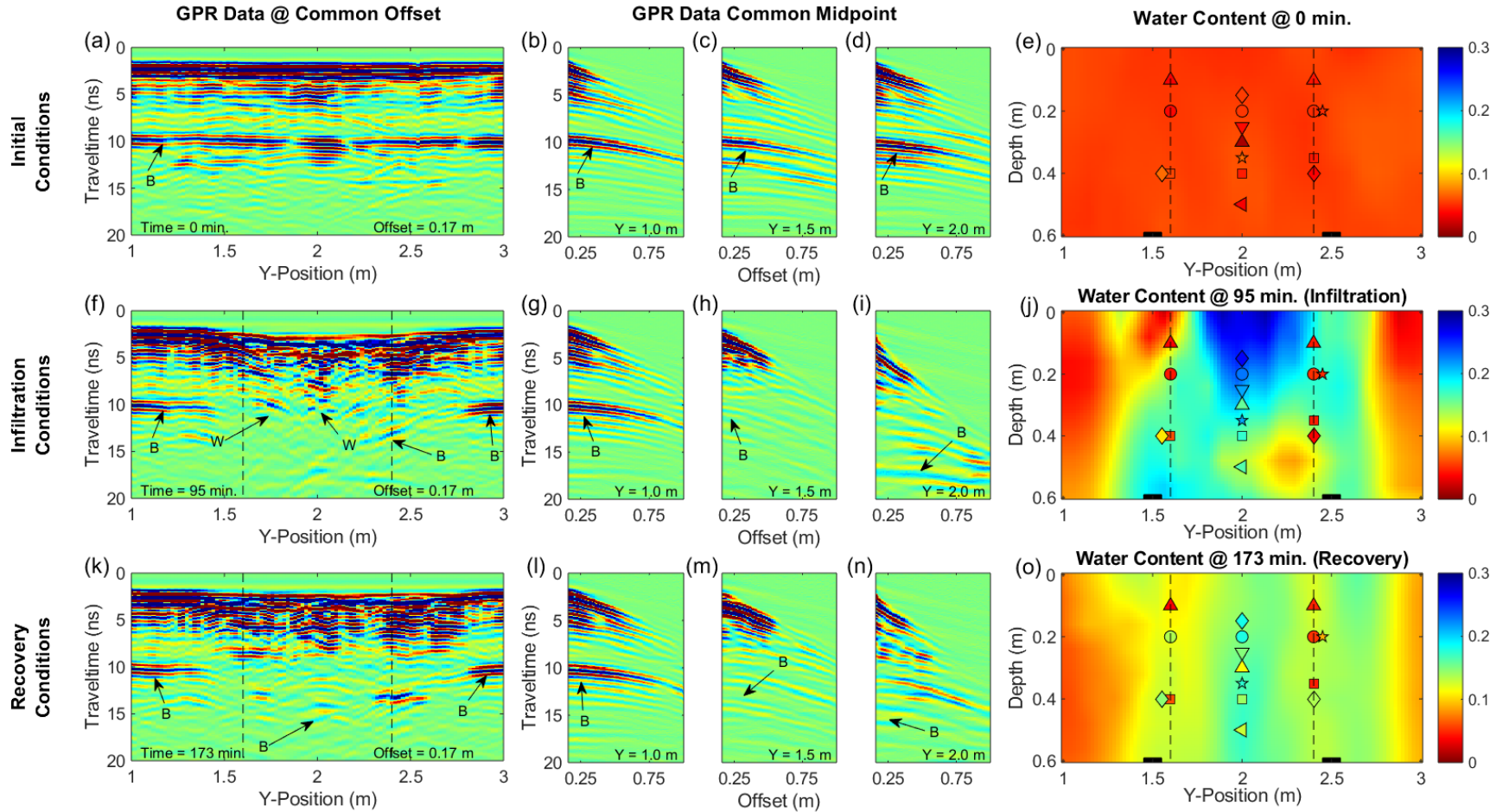
339 340 Figure 4: Panels (a, f, and k) are common-offset GPR data collected during the experiment. Panels (b-d, g-i, and l-n) are CMP data collected during the experiment. 341 Arrivals annotated are the sand layer reflection (B) and wetting front reflection (W). Panels (e, j, and o) show tomography results for the corresponding GPR data. 342 Vertical lines indicate the lateral extent of the wetted surface. Shapes correspond to the soil moisture data for the given y-location in Figure 5, colors correspond to 343 the measured soil moisture. Adjacent symbols are from probes that are located at different x-locations, but identical depths.
