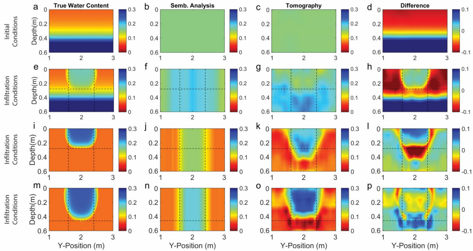
332 333 Figure 3: Panels (a), (e), (i), and (m) show true volumetric water content distributions from HYDRUS-2D. Panels (b), (f), (j), and (n) show starting models for the 334 tomography derived from semblance analysis. Panels (c), (g), (k), and (o) show results of tomography of the simulated GPR data as volumetric water content. 335 Difference plots (d), (h), (l), and (p) were calculated by subtracting the tomography results from the true water content distributions; red areas indicate volumetric 336 moisture overestimation while blue areas indicate volumetric moisture underestimation.
