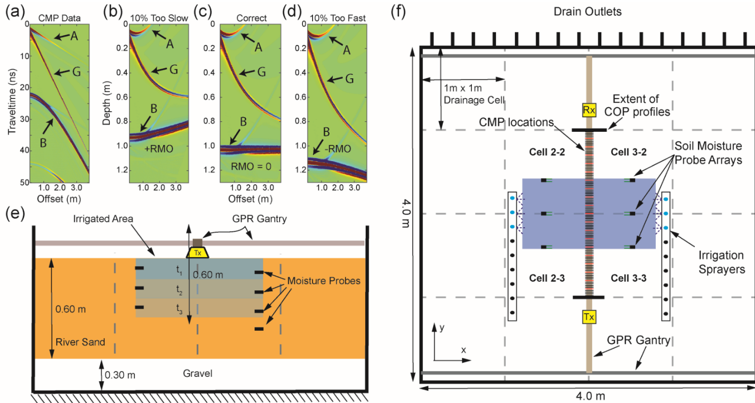
320 321 Figure 1: a) Example CMP data showing the airwave (A), groundwave (G) and reflection from a layer (B). Data in (a) is migrated to form (b) a migrated gather 322 with velocity 10% slow; c) a migrated gather with correct velocity; and d) a migrated gather with velocity 10% fast. Panel (e) shows a cross-section of the experiment 323 at y = 2.0 where t_1 , t_2 , and t_3 are arbitrary times during the infiltration. Panel (f) shows the plan-view of the experiment. Note that the bottom of the sand layer is 324 flat where GPR data collection occurs, i.e. on a boundary between drain cells, and pitched elsewhere toward cell drains.
