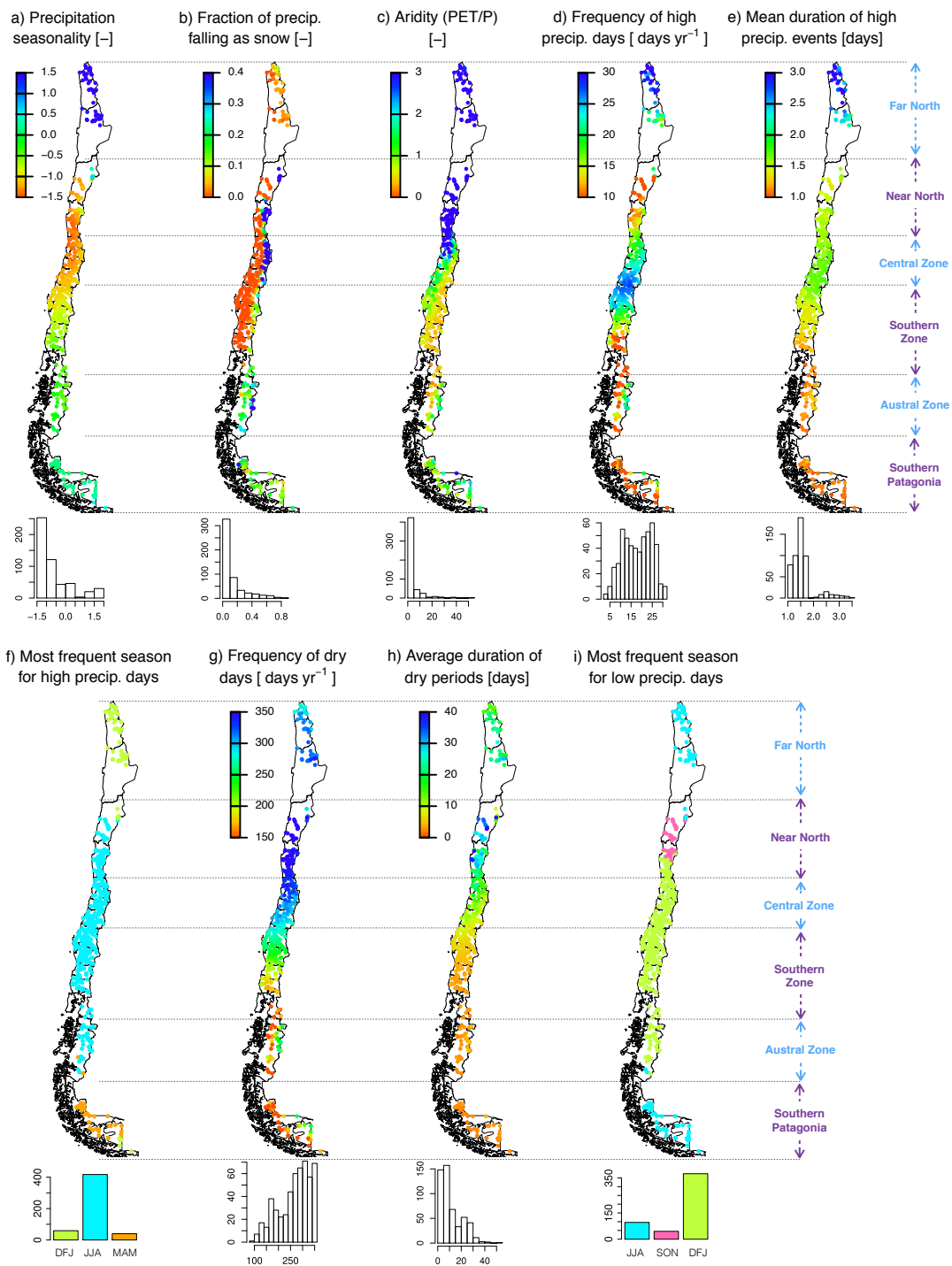
Figure 9: Climatic indices (calculated from precip cr2met product). The histograms indicate the number of catchments (out of 516) in each bin.
