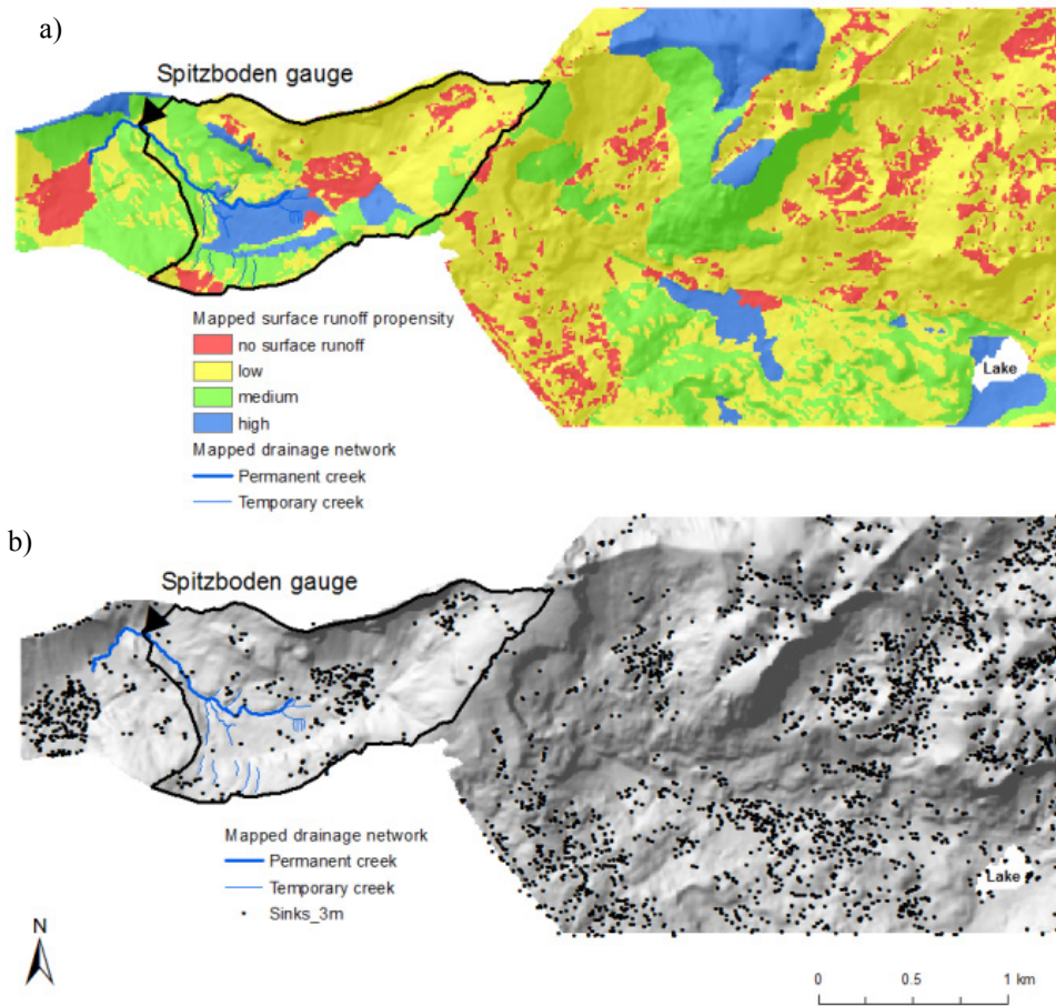
10 Figure 6: Comparison of the surface runoff propensity index (a) with sink holes (b). Sink holes have been automatically generated from the LiDAR terrain model at 3m resolution. Shading represents topography from the 1m terrain model. Black polygon shows the topographic catchment of the Spitzboden stream gauge.
