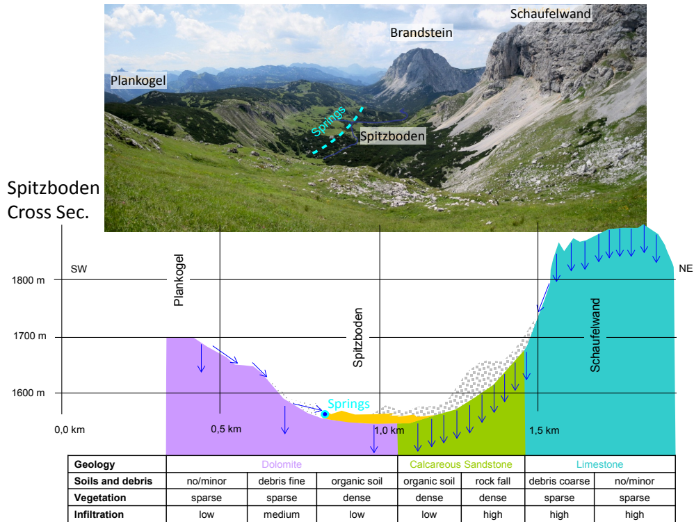
Figure 3: Cross section of the Spitzboden area illustrating the mapped properties (geology, soils and debris, vegetation and infiltration capacity, see Tab. 1). Yellow and grey shading relates to organic soil layer and coarse debris from the wall in the Northeast (NE), respectively. Blue arrows indicate dominant drainage directions during a typical summer storm; a higher density of arrows indicates larger fluxes.
