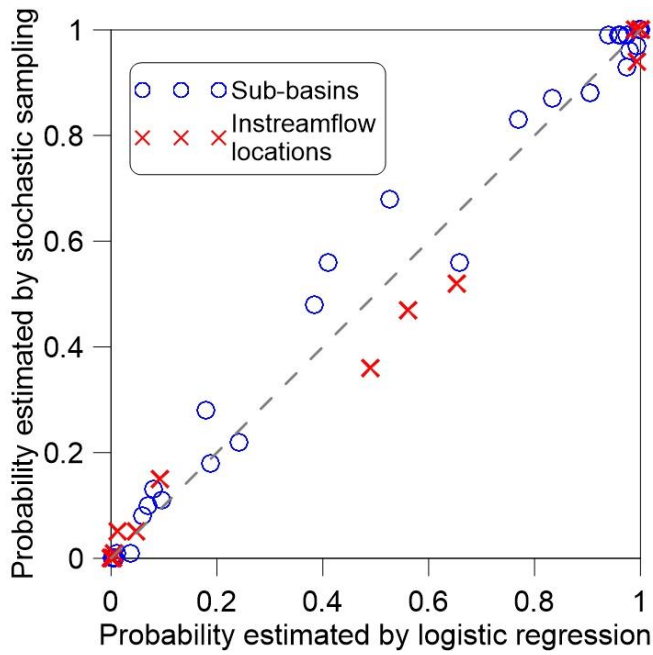
Figure 8: 1:1 plots between the probability estimates from the stochastic sampling and those from the logistic regressions for the case study. The probabilities of satisfactory performance at the 14 sub-basins and the 7 instream flow locations were estimated by the 100 Monte-Carlo simulations for each climatic perturbation. The number of points for comparison to the logistic models becomes 3 \text{ (perturbations)} \times 21 \text{ (locations)} = 63 .
