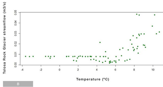
Fig. 2. Scatter plot of streamflow and mean daily air temperature for Horcones Inferior Glacier (A) and for Mt. Tolosa rock glaciers conglomerate (B).
