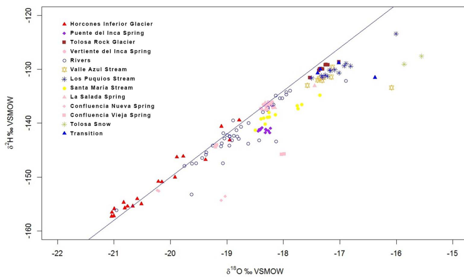
Fig. 3. \delta^{18}\text{O} and \delta^2\text{H} values scatter plot of the analyzed samples. The adjusted line is the global meteoric water line (Craig, 1961).
