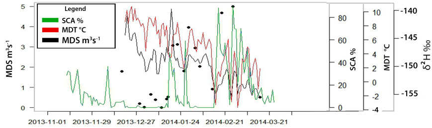
Fig. 4. Time-series showing the snow covered area (SCA), mean daily streamflow (MDS), mean daily air temperature (MDT) and \delta^2\text{H} composition of the Horcones Inferior Glacier (bold black dots).
