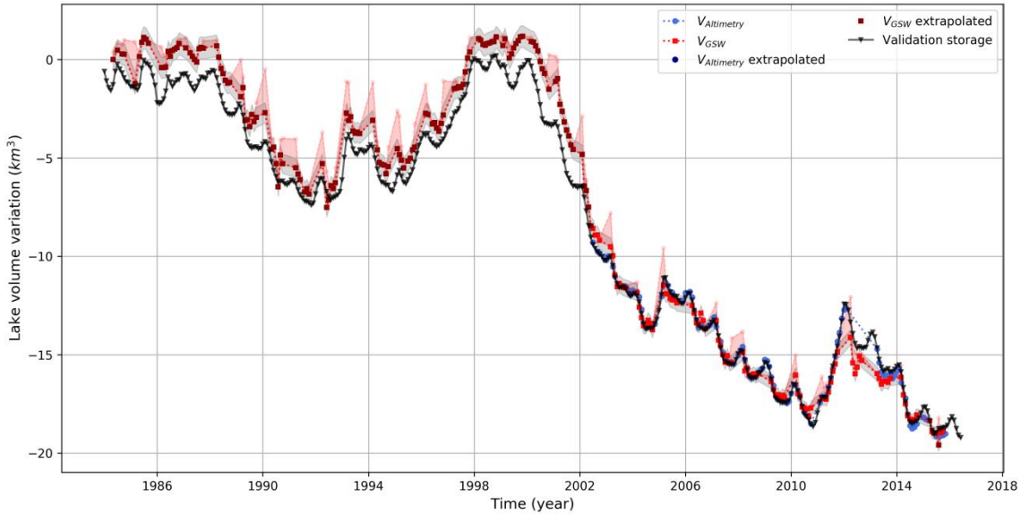
5 Figure 9 Validation time series plotted with estimated reservoir volumes for Lake Mead. The black triangle line represents the validation storage as measured using the full lake bathymetry. The grey and red shaded areas represent the 95 % residual-based CI and the uncertainty induced by the no data within MWE, respectively.
