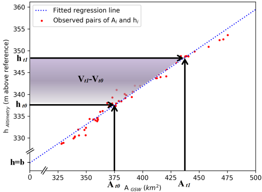
5 Figure 3 Volume variation calculation for Lake Mead. The observed monthly pairs of A and h (red dots) are used to estimate a linear regression (blue dashed line) that is used to calculate volumetric changes. The volumetric change from t_0 to t_1 is equal to the purple area and can be visually interpreted as a 2D lake section.
